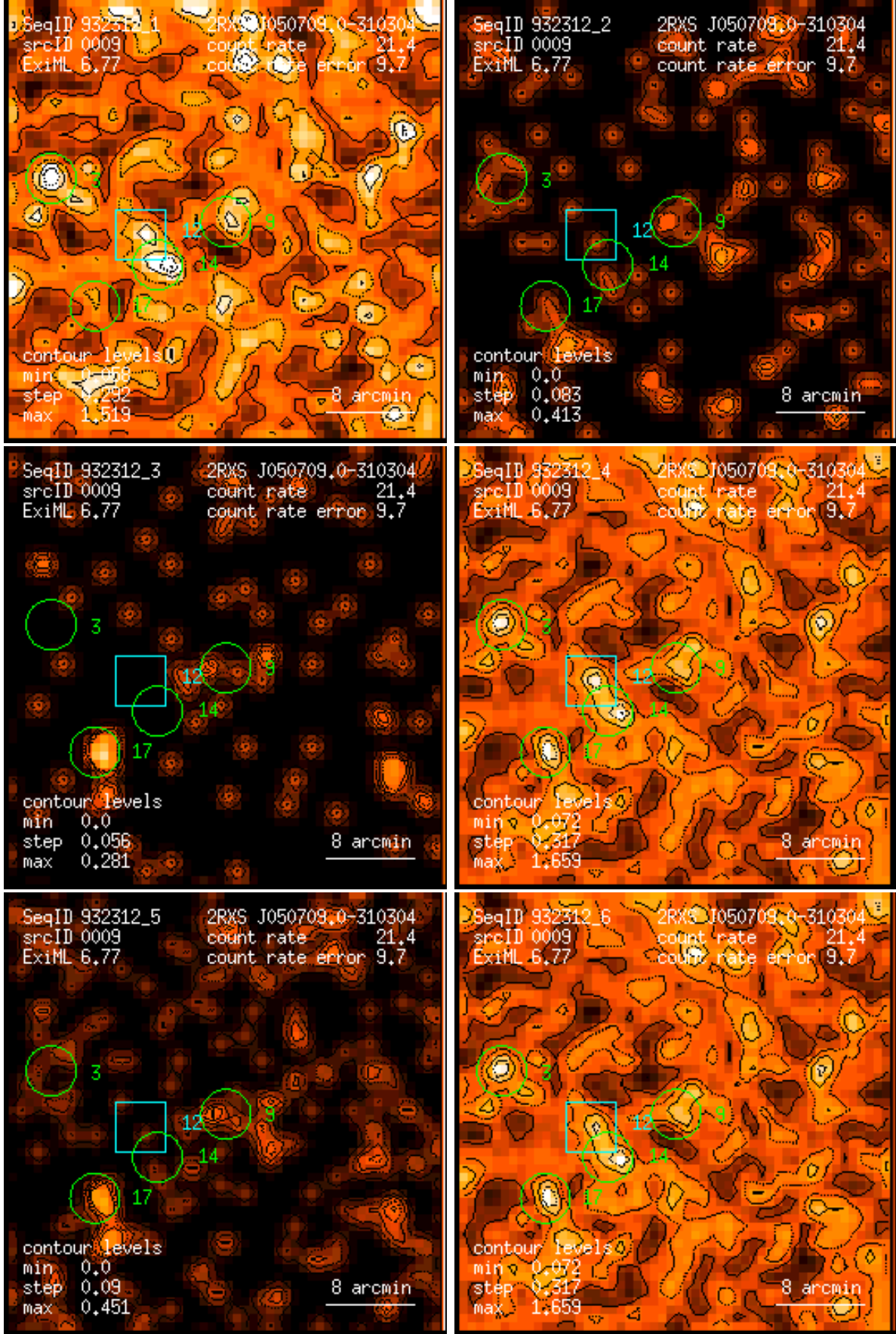
Figure 9: RASS 932312: detection 0009: band rate images, Gaussian filter: (1) PSPC channels 11 – 41, (2) 52 – 90, (3) 91 – 201, (4) 11 – 235, (5) 52 – 201, (6) 11 – 201. Broad band rates in counts/ks. Band rate contour levels in counts/ks/arcmin 2 .
