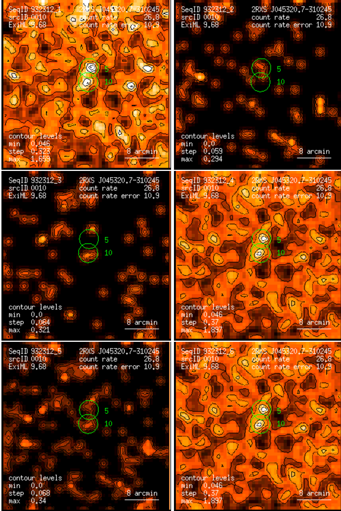
Figure 10: RASS 932312: detection 0010: band rate images, Gaussian filter: (1) PSPC channels 11 – 41, (2) 52 – 90, (3) 91 – 201, (4) 11 – 235, (5) 52 – 201, (6) 11 – 201. Broad band rates in counts/ks. Band rate contour levels in counts/ks/arcmin 2 .
