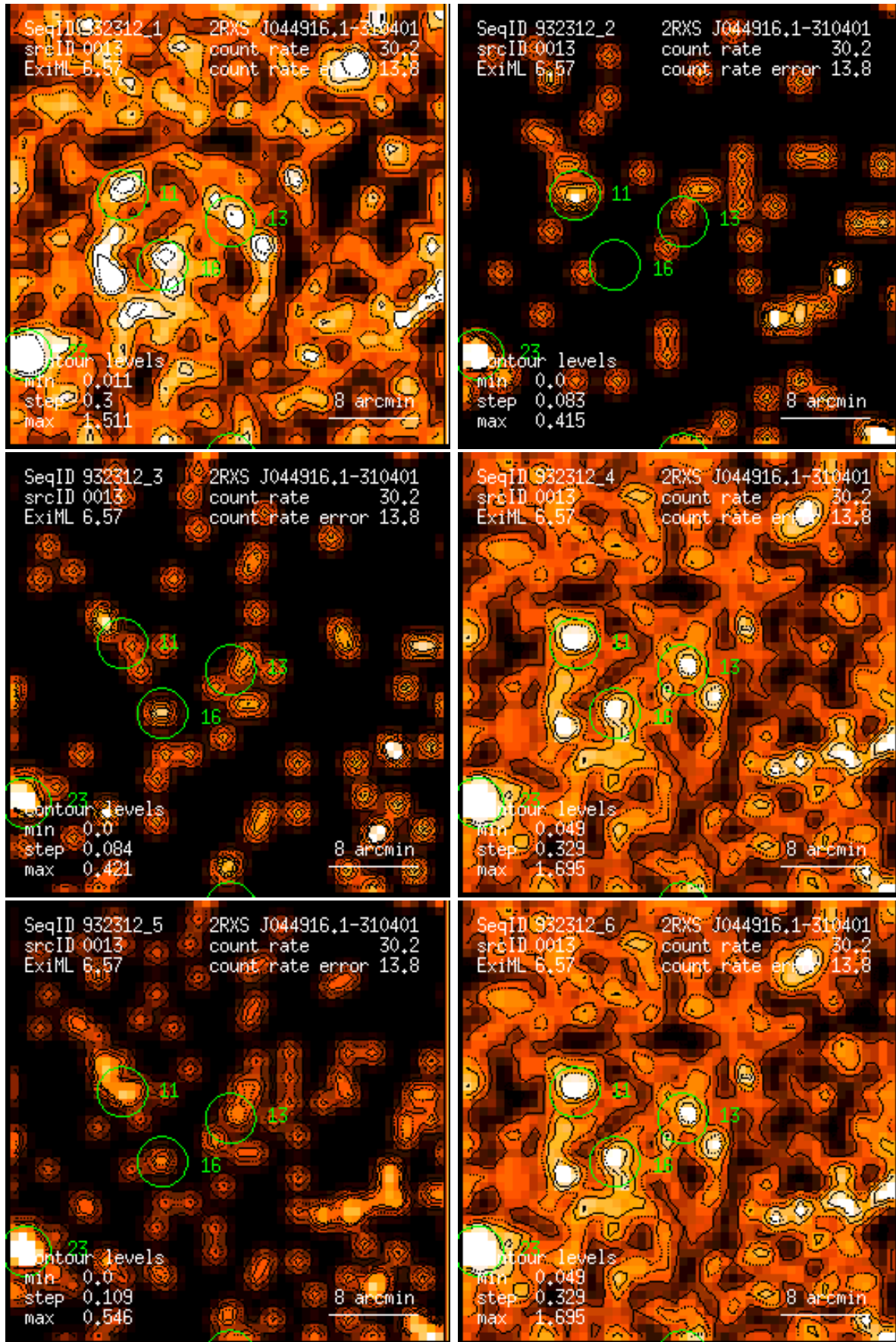
Figure 13: RASS 932312: detection 0013: band rate images, Gaussian filter: (1) PSPC channels 11 – 41, (2) 52 – 90, (3) 91 – 201, (4) 11 – 235, (5) 52 – 201, (6) 11 – 201. Broad band rates in counts/ks. Band rate contour levels in counts/ks/arcmin 2 .
