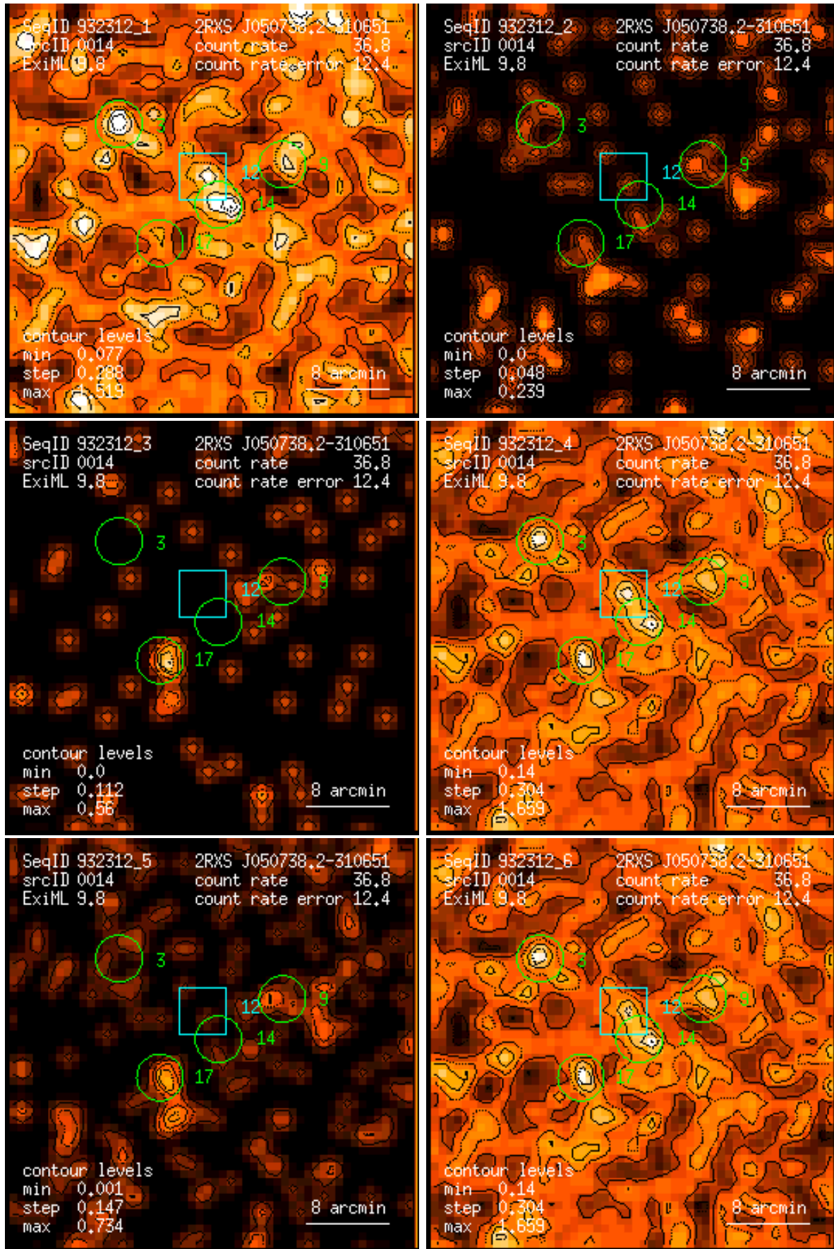
Figure 14: RASS 932312: detection 0014: band rate images, Gaussian filter: (1) PSPC channels 11 – 41, (2) 52 – 90, (3) 91 – 201, (4) 11 – 235, (5) 52 – 201, (6) 11 – 201. Broad band rates in counts/ks. Band rate contour levels in counts/ks/arcmin 2 .
