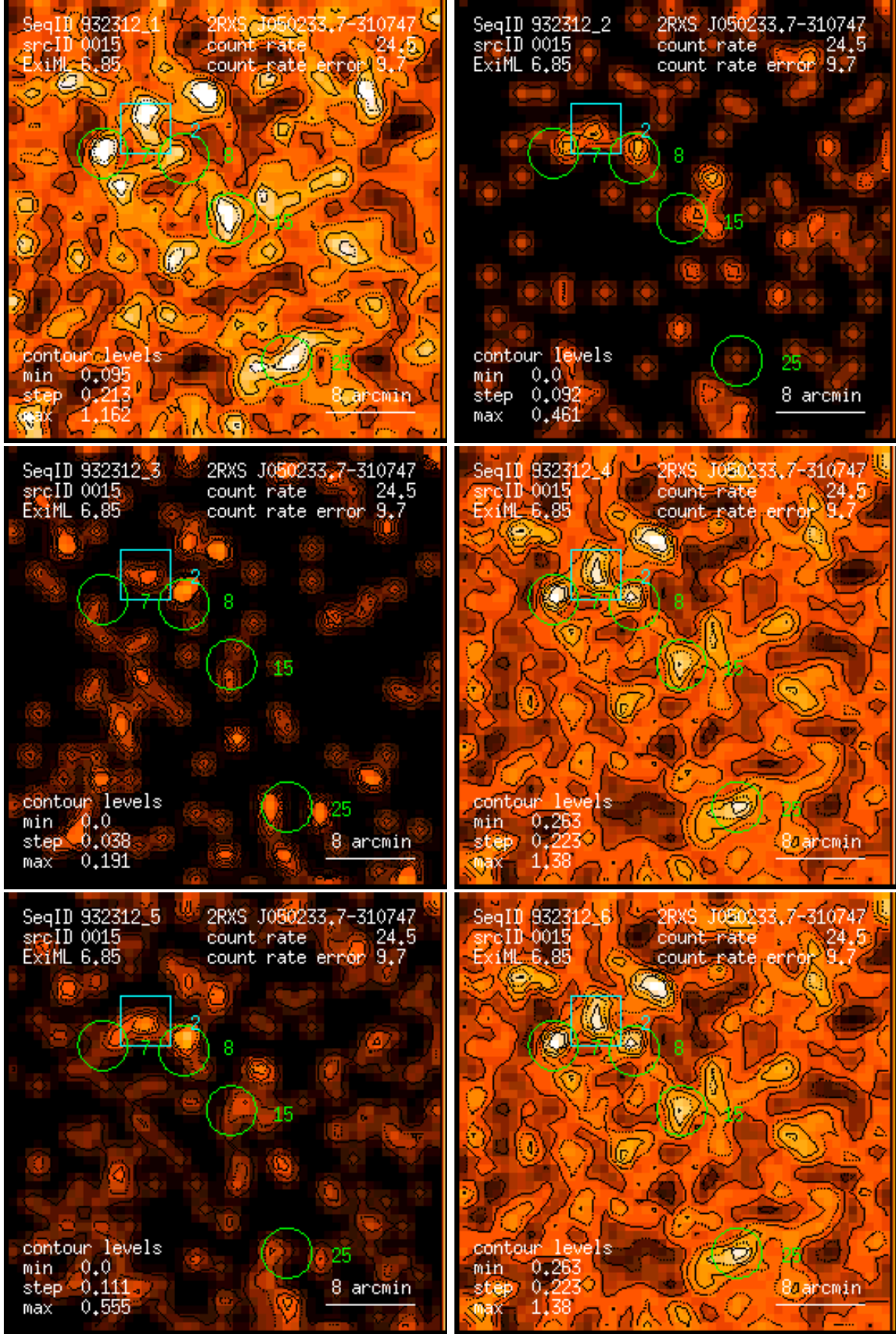
Figure 15: RASS 932312: detection 0015: band rate images, Gaussian filter: (1) PSPC channels 11 – 41, (2) 52 – 90, (3) 91 – 201, (4) 11 – 235, (5) 52 – 201, (6) 11 – 201. Broad band rates in counts/ks. Band rate contour levels in counts/ks/arcmin 2 .
