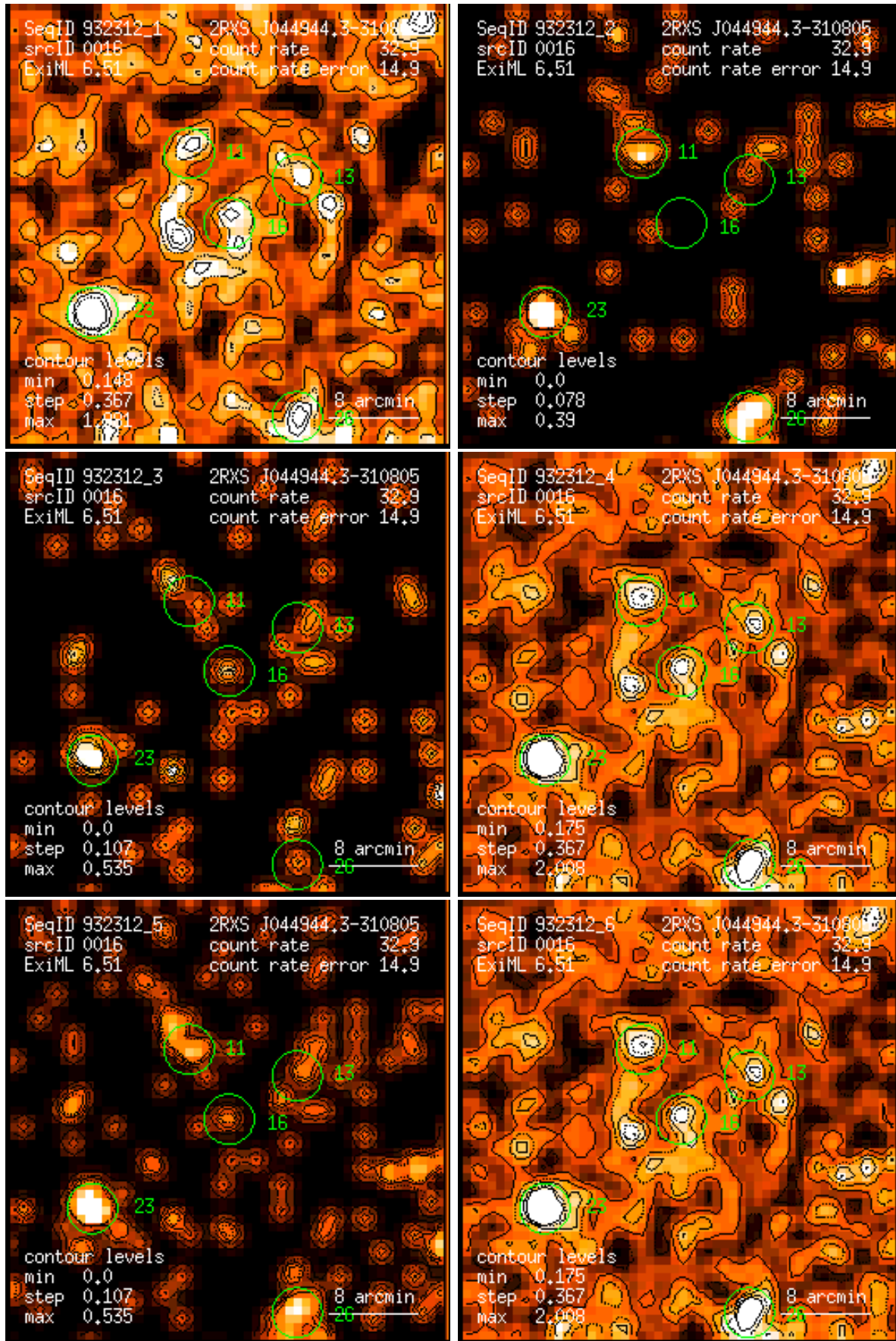
Figure 16: RASS 932312: detection 0016: band rate images, Gaussian filter: (1) PSPC channels 11 – 41, (2) 52 – 90, (3) 91 – 201, (4) 11 – 235, (5) 52 – 201, (6) 11 – 201. Broad band rates in counts/ks. Band rate contour levels in counts/ks/arcmin 2 .
