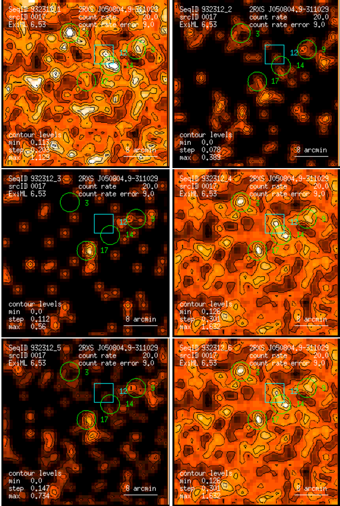
Figure 17: RASS 932312: detection 0017: band rate images, Gaussian filter: (1) PSPC channels 11 – 41, (2) 52 – 90, (3) 91 – 201, (4) 11 – 235, (5) 52 – 201, (6) 11 – 201. Broad band rates in counts/ks. Band rate contour levels in counts/ks/arcmin 2 .
