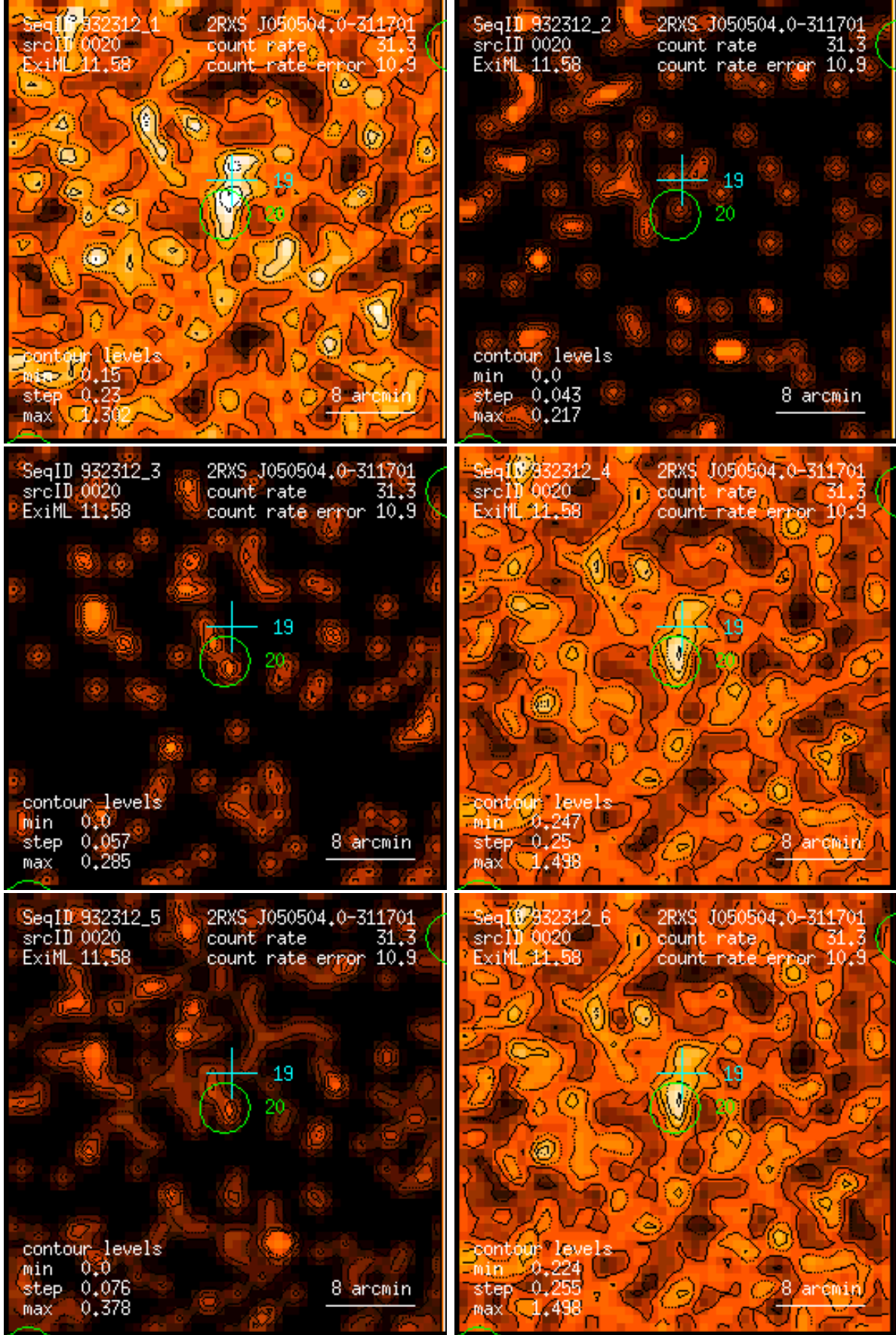
Figure 20: RASS 932312: detection 0020: band rate images, Gaussian filter: (1) PSPC channels 11 – 41, (2) 52 – 90, (3) 91 – 201, (4) 11 – 235, (5) 52 – 201, (6) 11 – 201. Broad band rates in counts/ks. Band rate contour levels in counts/ks/arcmin 2 .
