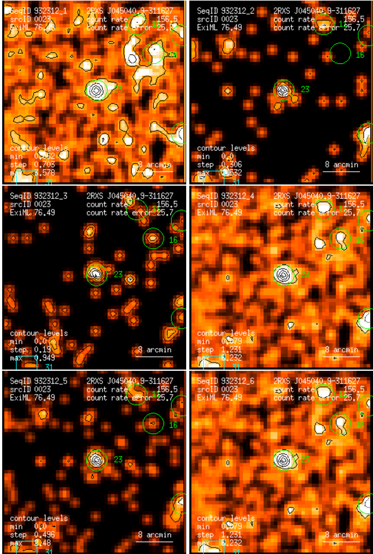
Figure 23: RASS 932312: detection 0023: band rate images, Gaussian filter: (1) PSPC channels 11 – 41, (2) 52 – 90, (3) 91 – 201, (4) 11 – 235, (5) 52 – 201, (6) 11 – 201. Broad band rates in counts/ks. Band rate contour levels in counts/ks/arcmin 2 .
