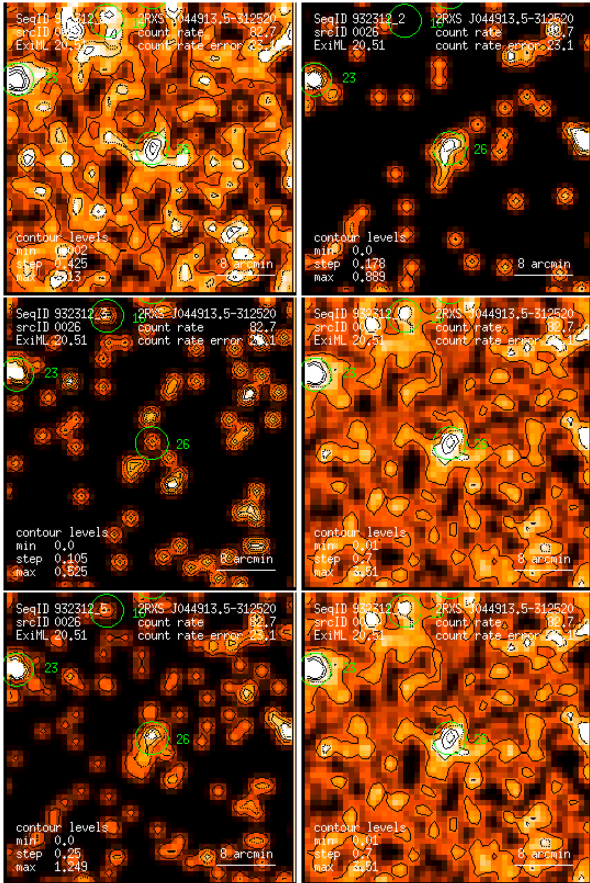
Figure 26: RASS 932312: detection 0026: band rate images, Gaussian filter: (1) PSPC channels 11 – 41, (2) 52 – 90, (3) 91 – 201, (4) 11 – 235, (5) 52 – 201, (6) 11 – 201. Broad band rates in counts/ks. Band rate contour levels in counts/ks/arcmin 2 .
