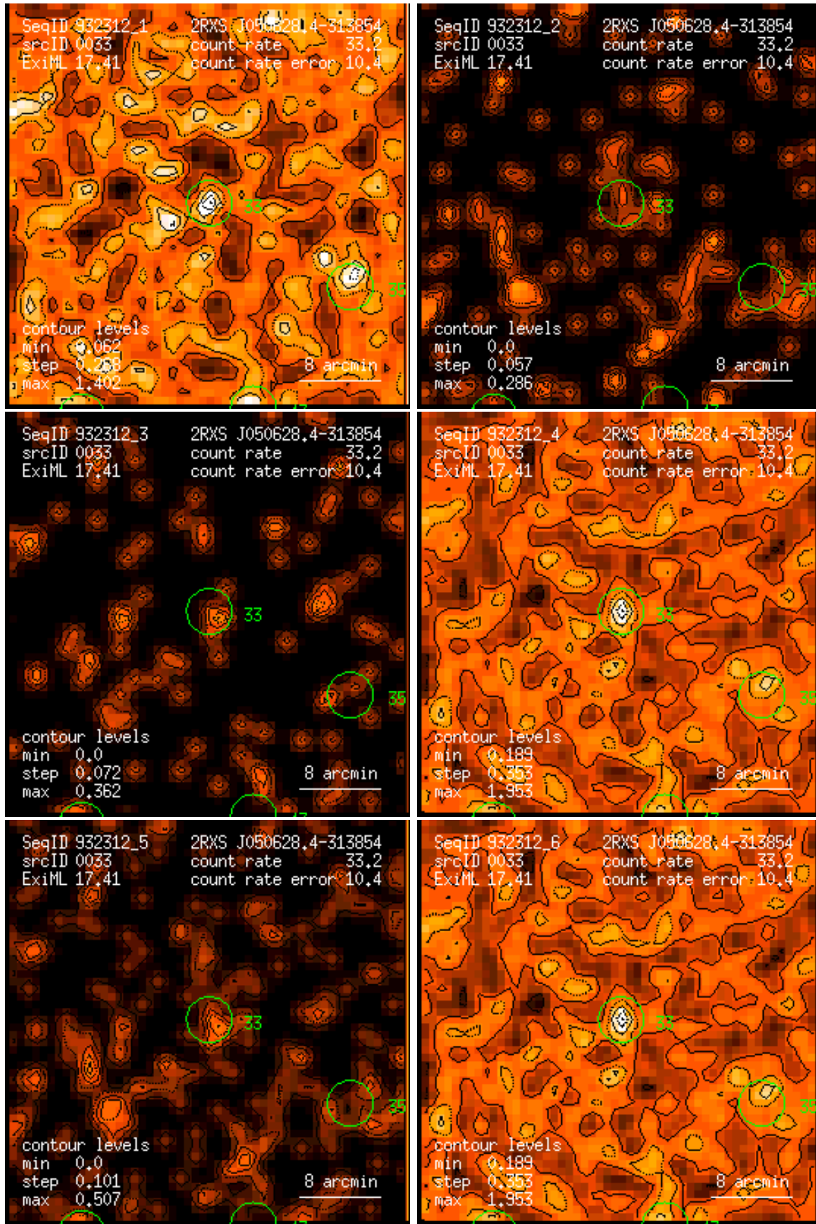
Figure 33: RASS 932312: detection 0033: band rate images, Gaussian filter: (1) PSPC channels 11 – 41, (2) 52 – 90, (3) 91 – 201, (4) 11 – 235, (5) 52 – 201, (6) 11 – 201. Broad band rates in counts/ks. Band rate contour levels in counts/ks/arcmin 2 .
