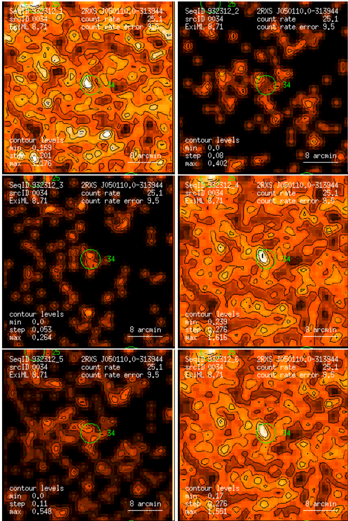
Figure 34: RASS 932312: detection 0034: band rate images, Gaussian filter: (1) PSPC channels 11 – 41, (2) 52 – 90, (3) 91 – 201, (4) 11 – 235, (5) 52 – 201, (6) 11 – 201. Broad band rates in counts/ks. Band rate contour levels in counts/ks/arcmin 2 .
