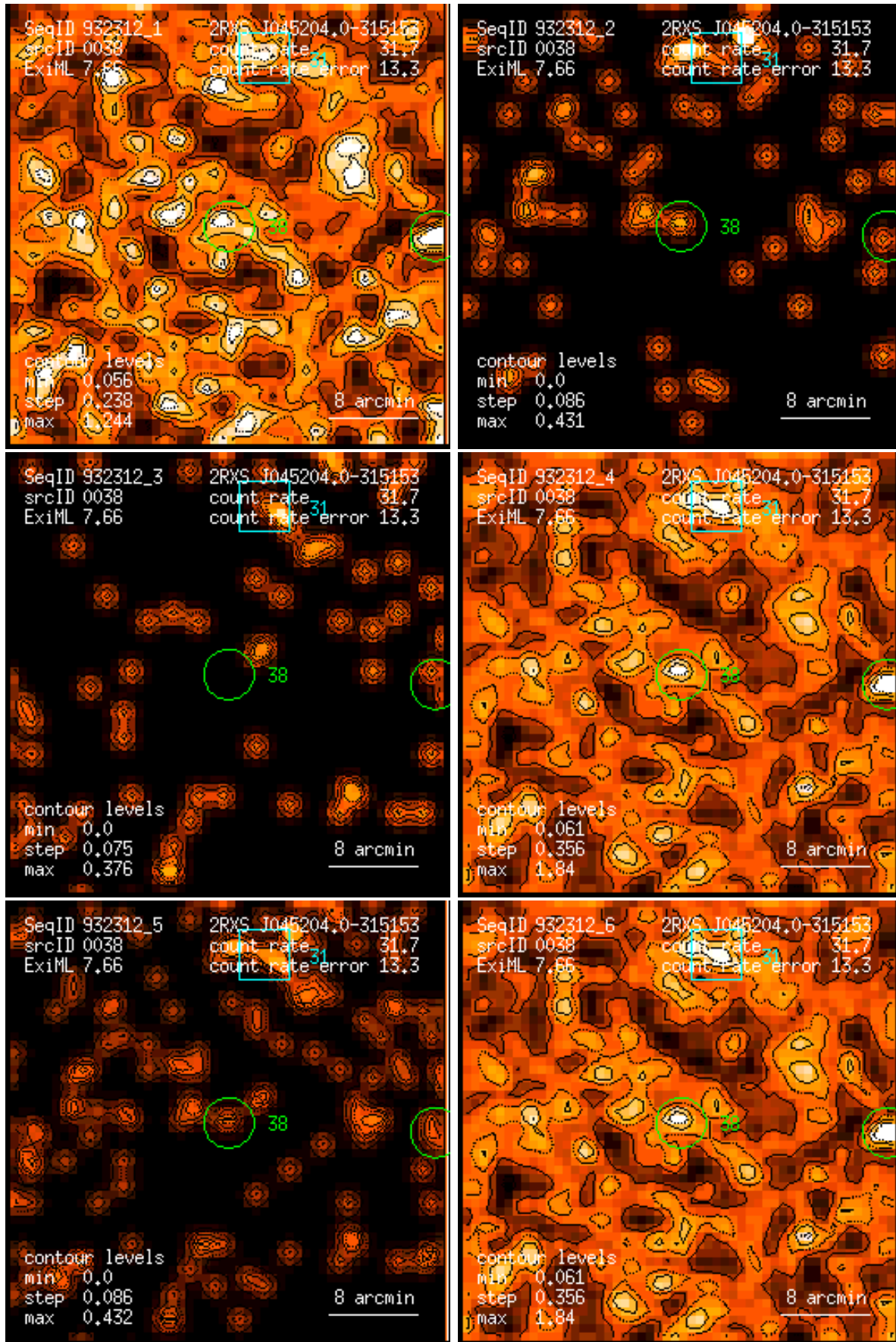
Figure 38: RASS 932312: detection 0038: band rate images, Gaussian filter: (1) PSPC channels 11 – 41, (2) 52 – 90, (3) 91 – 201, (4) 11 – 235, (5) 52 – 201, (6) 11 – 201. Broad band rates in counts/ks. Band rate contour levels in counts/ks/arcmin 2 .
