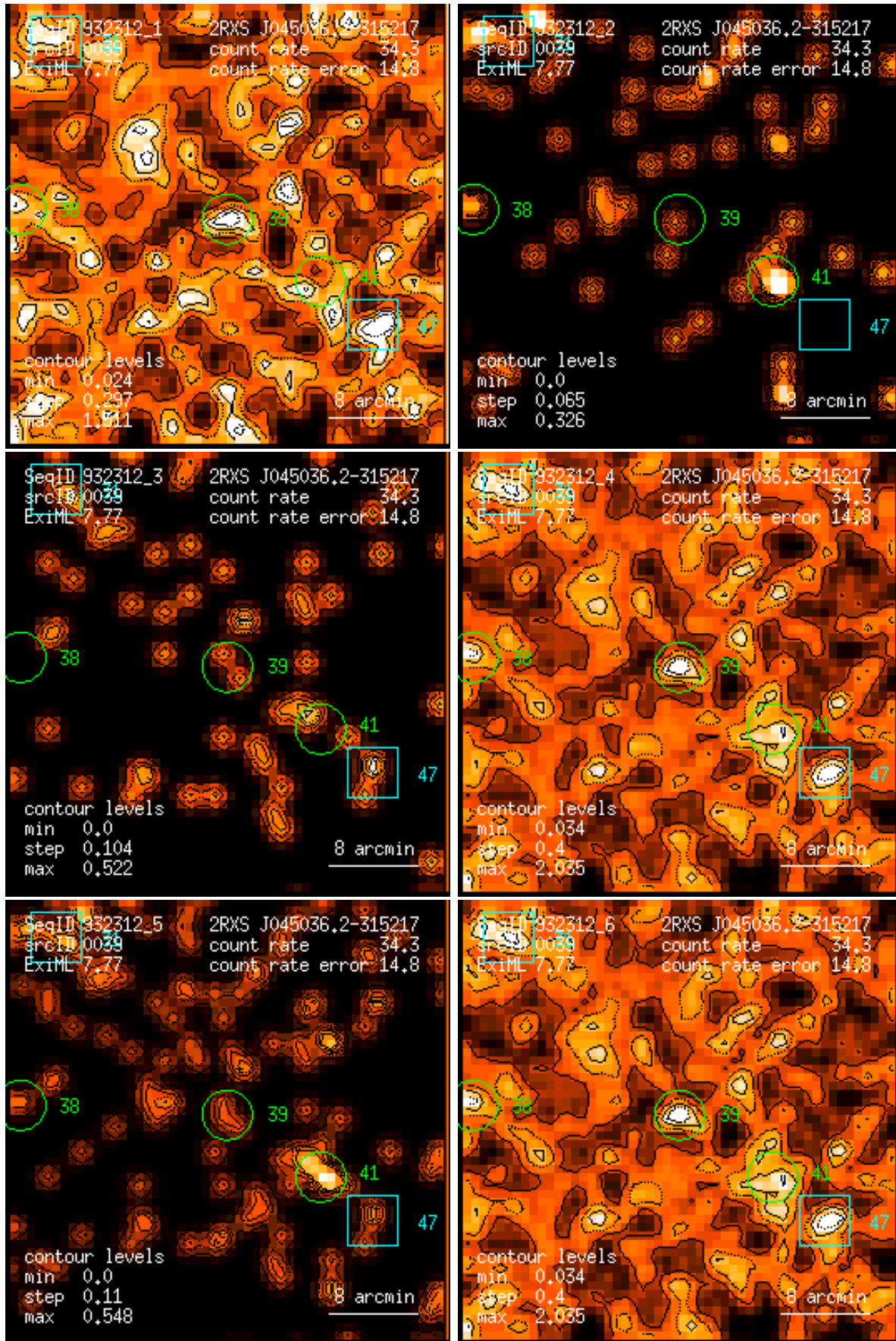
Figure 39: RASS 932312: detection 0039: band rate images, Gaussian filter: (1) PSPC channels 11 – 41, (2) 52 – 90, (3) 91 – 201, (4) 11 – 235, (5) 52 – 201, (6) 11 – 201. Broad band rates in counts/ks. Band rate contour levels in counts/ks/arcmin 2 .
