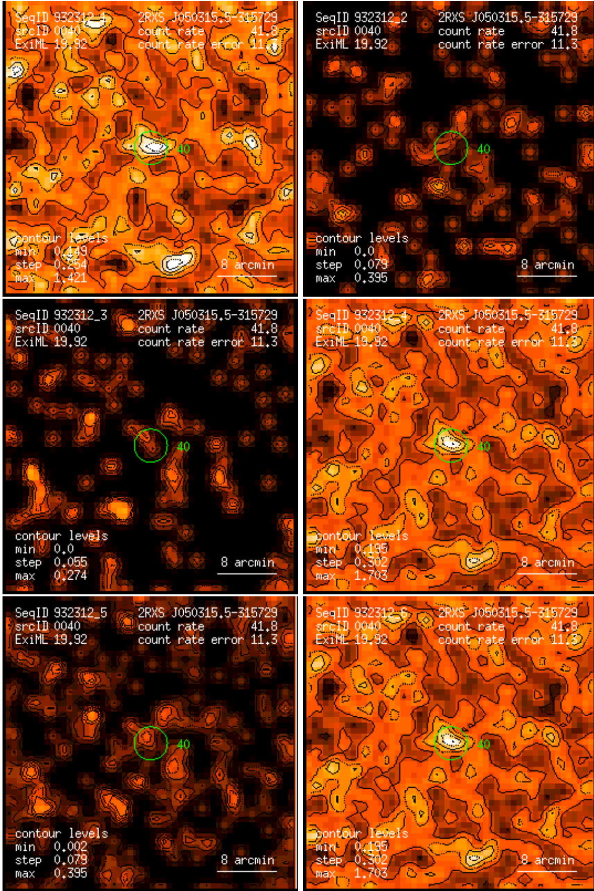
Figure 40: RASS 932312: detection 0040: band rate images, Gaussian filter: (1) PSPC channels 11 – 41, (2) 52 – 90, (3) 91 – 201, (4) 11 – 235, (5) 52 – 201, (6) 11 – 201. Broad band rates in counts/ks. Band rate contour levels in counts/ks/arcmin 2 .
