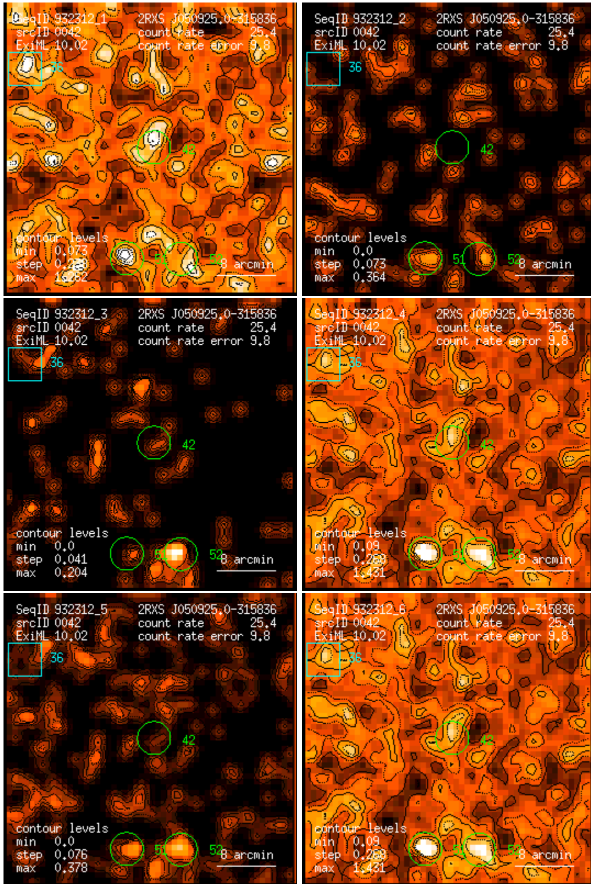
Figure 42: RASS 932312: detection 0042: band rate images, Gaussian filter: (1) PSPC channels 11 – 41, (2) 52 – 90, (3) 91 – 201, (4) 11 – 235, (5) 52 – 201, (6) 11 – 201. Broad band rates in counts/ks. Band rate contour levels in counts/ks/arcmin 2 .
