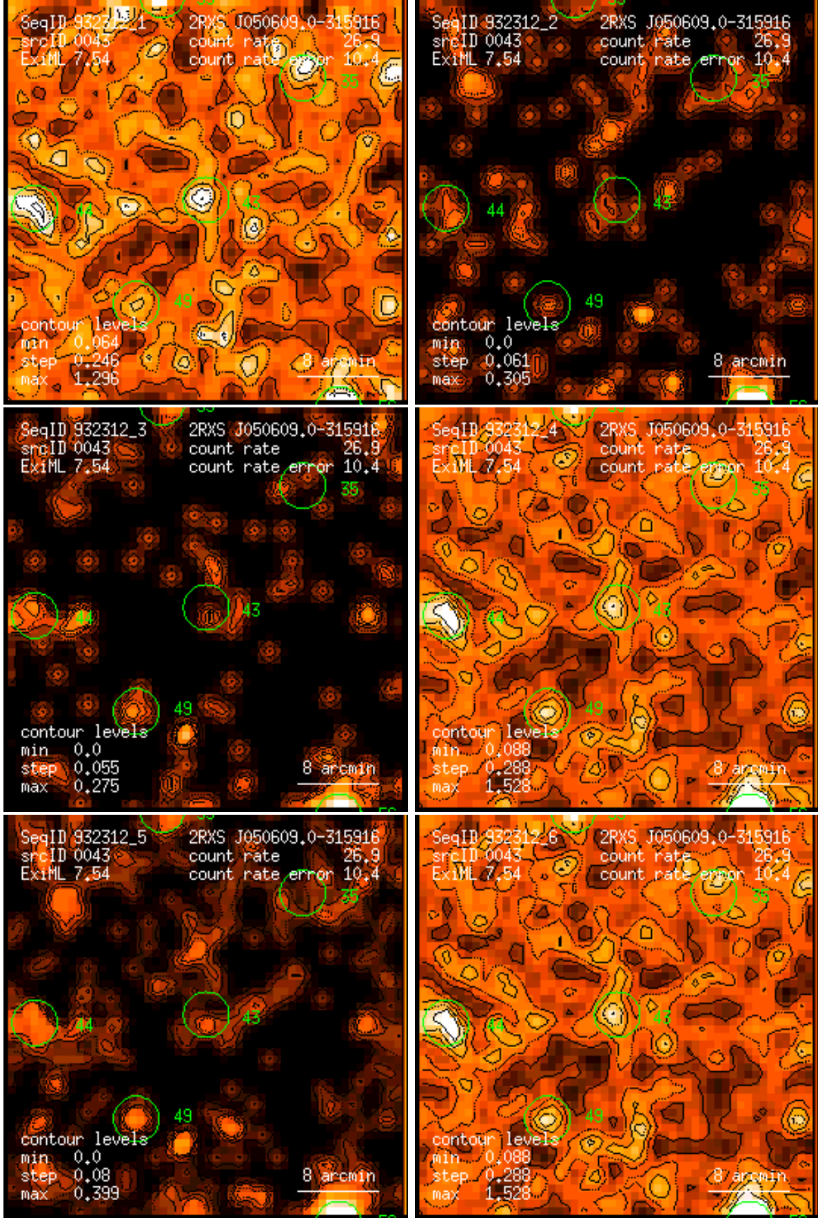
Figure 43: RASS 932312: detection 0043: band rate images, Gaussian filter: (1) PSPC channels 11 – 41, (2) 52 – 90, (3) 91 – 201, (4) 11 – 235, (5) 52 – 201, (6) 11 – 201. Broad band rates in counts/ks. Band rate contour levels in counts/ks/arcmin 2 .
