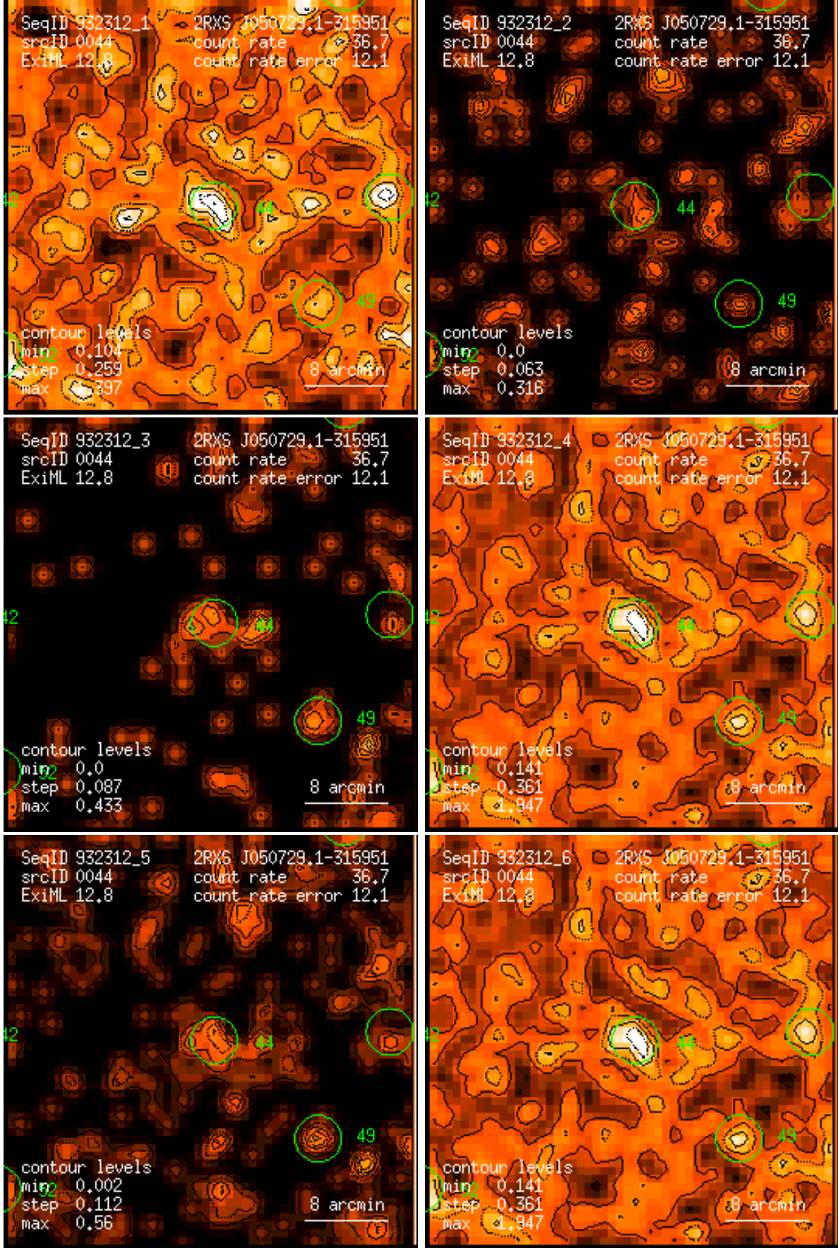
Figure 44: RASS 932312: detection 0044: band rate images, Gaussian filter: (1) PSPC channels 11 – 41, (2) 52 – 90, (3) 91 – 201, (4) 11 – 235, (5) 52 – 201, (6) 11 – 201. Broad band rates in counts/ks. Band rate contour levels in counts/ks/arcmin 2 .
