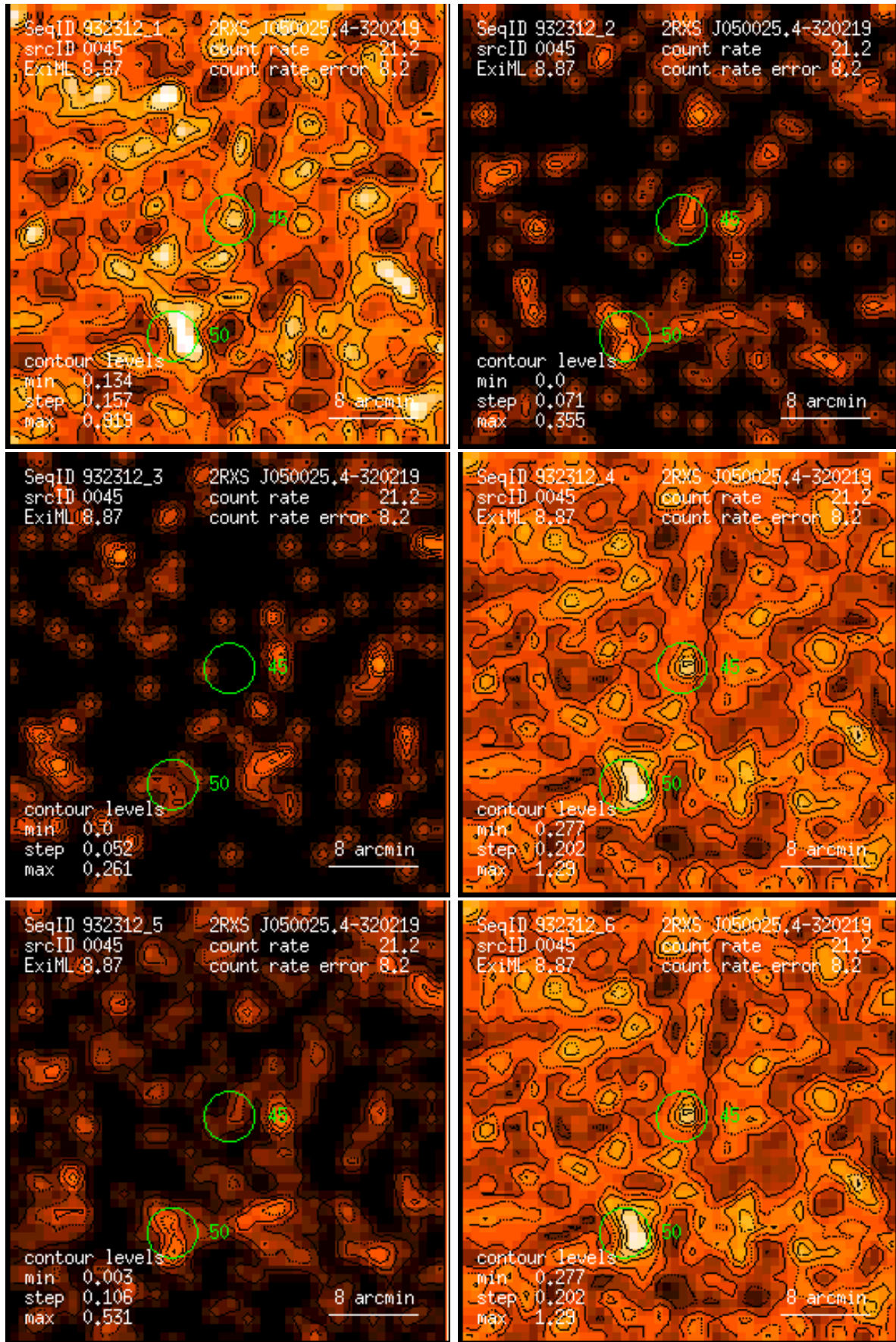
Figure 45: RASS 932312: detection 0045: band rate images, Gaussian filter: (1) PSPC channels 11 – 41, (2) 52 – 90, (3) 91 – 201, (4) 11 – 235, (5) 52 – 201, (6) 11 – 201. Broad band rates in counts/ks. Band rate contour levels in counts/ks/arcmin 2 .
