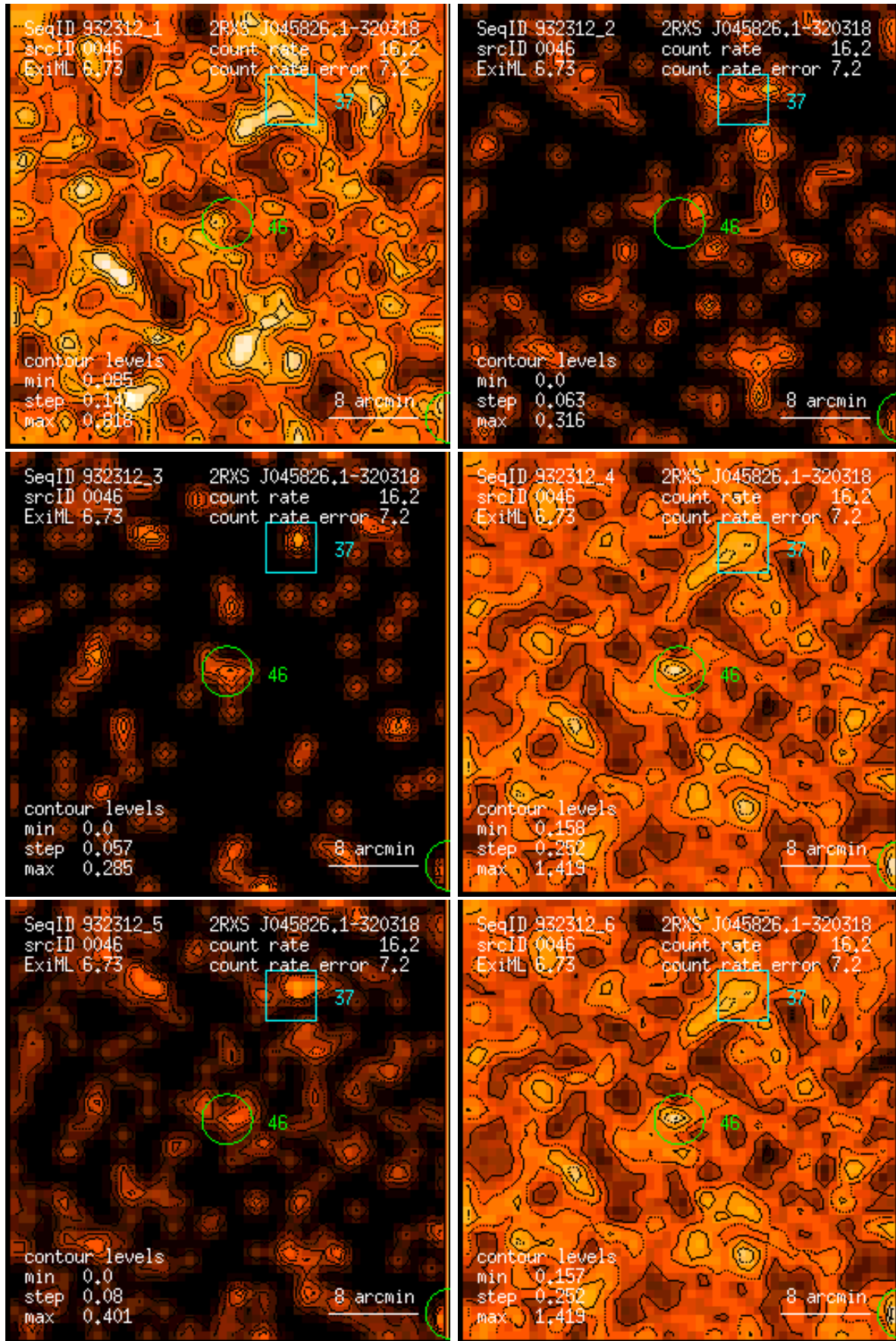
Figure 46: RASS 932312: detection 0046: band rate images, Gaussian filter: (1) PSPC channels 11 – 41, (2) 52 – 90, (3) 91 – 201, (4) 11 – 235, (5) 52 – 201, (6) 11 – 201. Broad band rates in counts/ks. Band rate contour levels in counts/ks/arcmin 2 .
