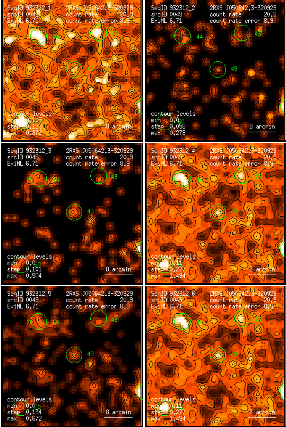
Figure 49: RASS 932312: detection 0049: band rate images, Gaussian filter: (1) PSPC channels 11 – 41, (2) 52 – 90, (3) 91 – 201, (4) 11 – 235, (5) 52 – 201, (6) 11 – 201. Broad band rates in counts/ks. Band rate contour levels in counts/ks/arcmin 2 .
