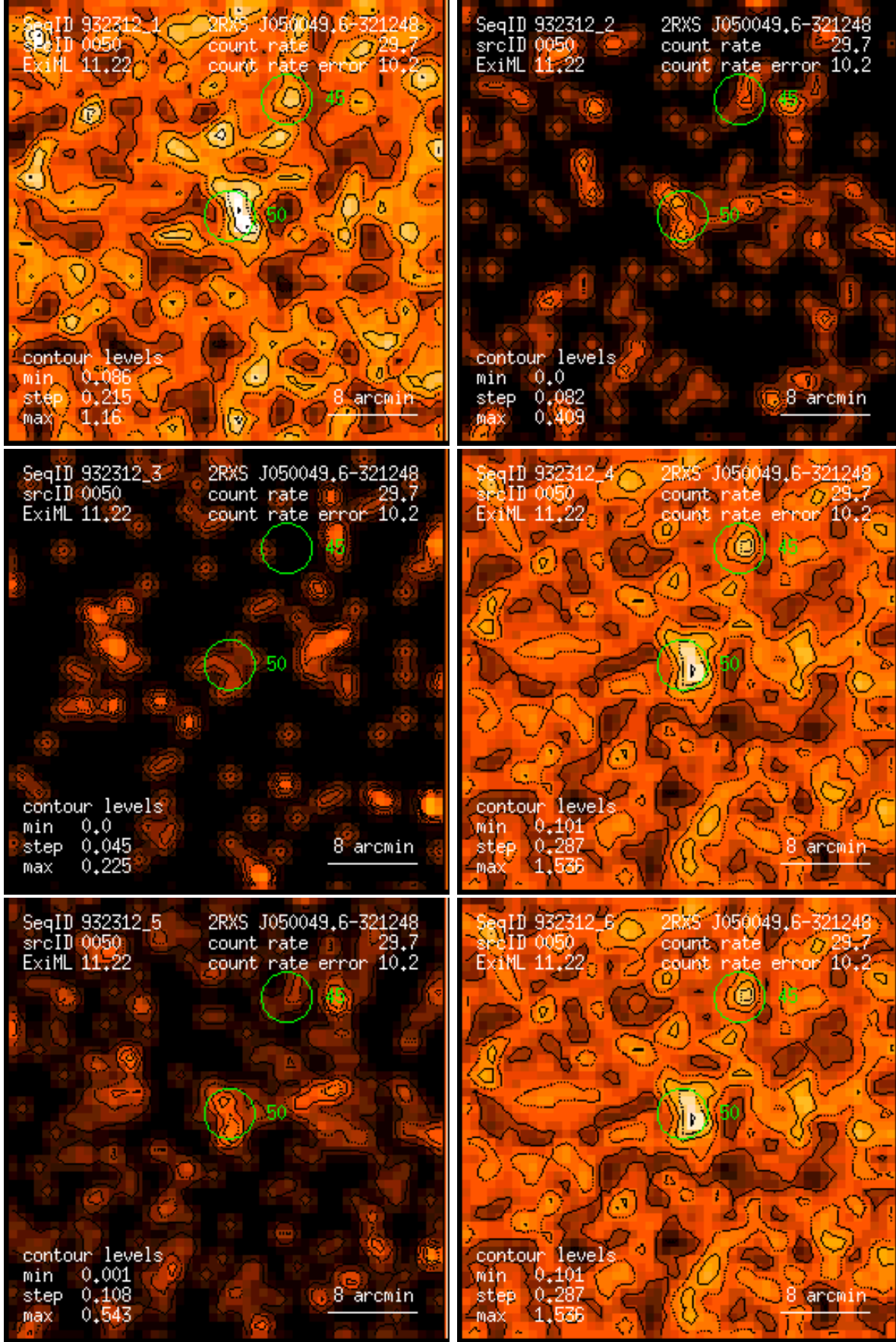
Figure 50: RASS 932312: detection 0050: band rate images, Gaussian filter: (1) PSPC channels 11 – 41, (2) 52 – 90, (3) 91 – 201, (4) 11 – 235, (5) 52 – 201, (6) 11 – 201. Broad band rates in counts/ks. Band rate contour levels in counts/ks/arcmin 2 .
