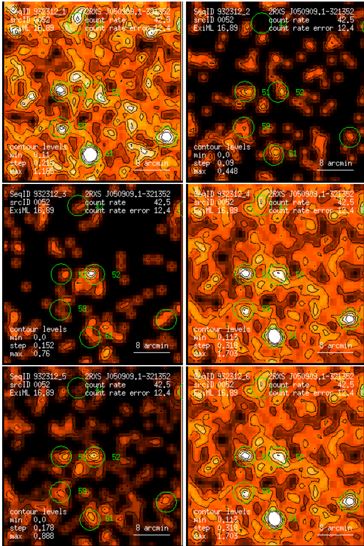
Figure 52: RASS 932312: detection 0052: band rate images, Gaussian filter: (1) PSPC channels 11 – 41, (2) 52 – 90, (3) 91 – 201, (4) 11 – 235, (5) 52 – 201, (6) 11 – 201. Broad band rates in counts/ks. Band rate contour levels in counts/ks/arcmin 2 .
