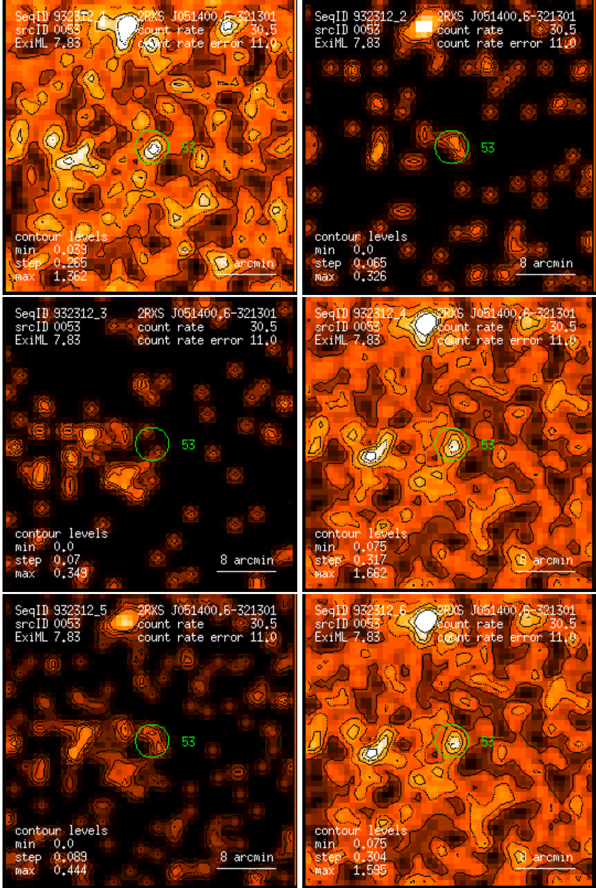
Figure 53: RASS 932312: detection 0053: band rate images, Gaussian filter: (1) PSPC channels 11 – 41, (2) 52 – 90, (3) 91 – 201, (4) 11 – 235, (5) 52 – 201, (6) 11 – 201. Broad band rates in counts/ks. Band rate contour levels in counts/ks/arcmin 2 .
