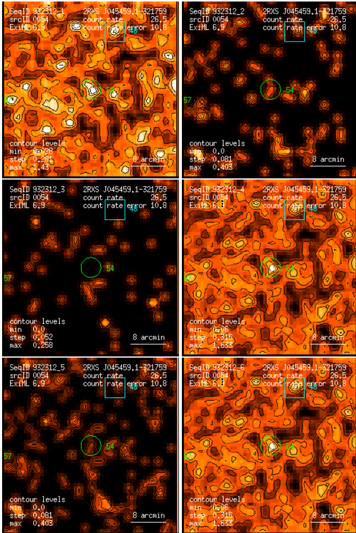
Figure 54: RASS 932312: detection 0054: band rate images, Gaussian filter: (1) PSPC channels 11 – 41, (2) 52 – 90, (3) 91 – 201, (4) 11 – 235, (5) 52 – 201, (6) 11 – 201. Broad band rates in counts/ks. Band rate contour levels in counts/ks/arcmin 2 .
