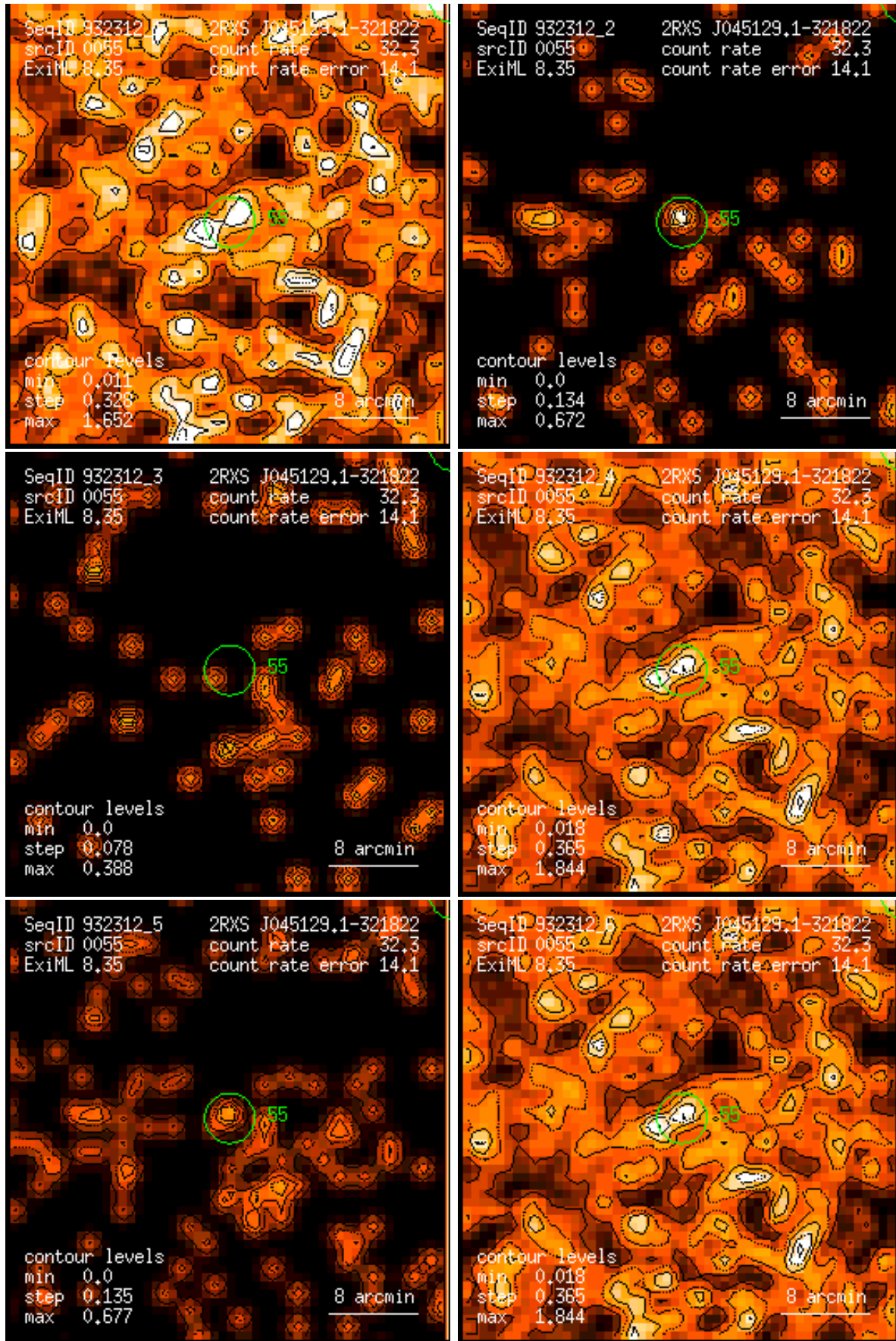
Figure 55: RASS 932312: detection 0055: band rate images, Gaussian filter: (1) PSPC channels 11 – 41, (2) 52 – 90, (3) 91 – 201, (4) 11 – 235, (5) 52 – 201, (6) 11 – 201. Broad band rates in counts/ks. Band rate contour levels in counts/ks/arcmin 2 .
