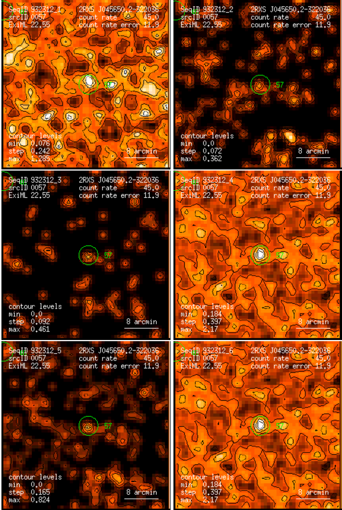
Figure 57: RASS 932312: detection 0057: band rate images, Gaussian filter: (1) PSPC channels 11 – 41, (2) 52 – 90, (3) 91 – 201, (4) 11 – 235, (5) 52 – 201, (6) 11 – 201. Broad band rates in counts/ks. Band rate contour levels in counts/ks/arcmin 2 .
