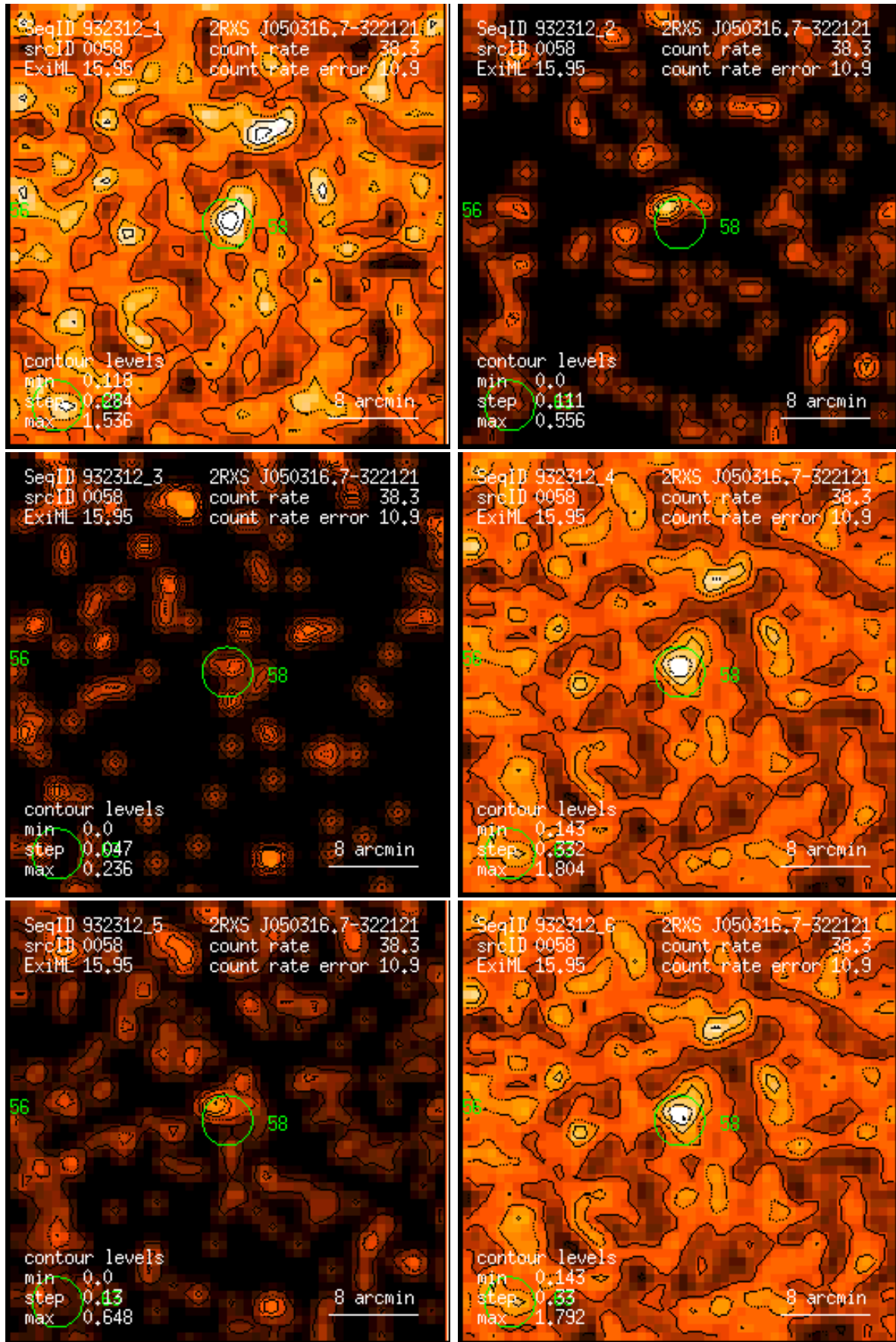
Figure 58: RASS 932312: detection 0058: band rate images, Gaussian filter: (1) PSPC channels 11 – 41, (2) 52 – 90, (3) 91 – 201, (4) 11 – 235, (5) 52 – 201, (6) 11 – 201. Broad band rates in counts/ks. Band rate contour levels in counts/ks/arcmin 2 .
