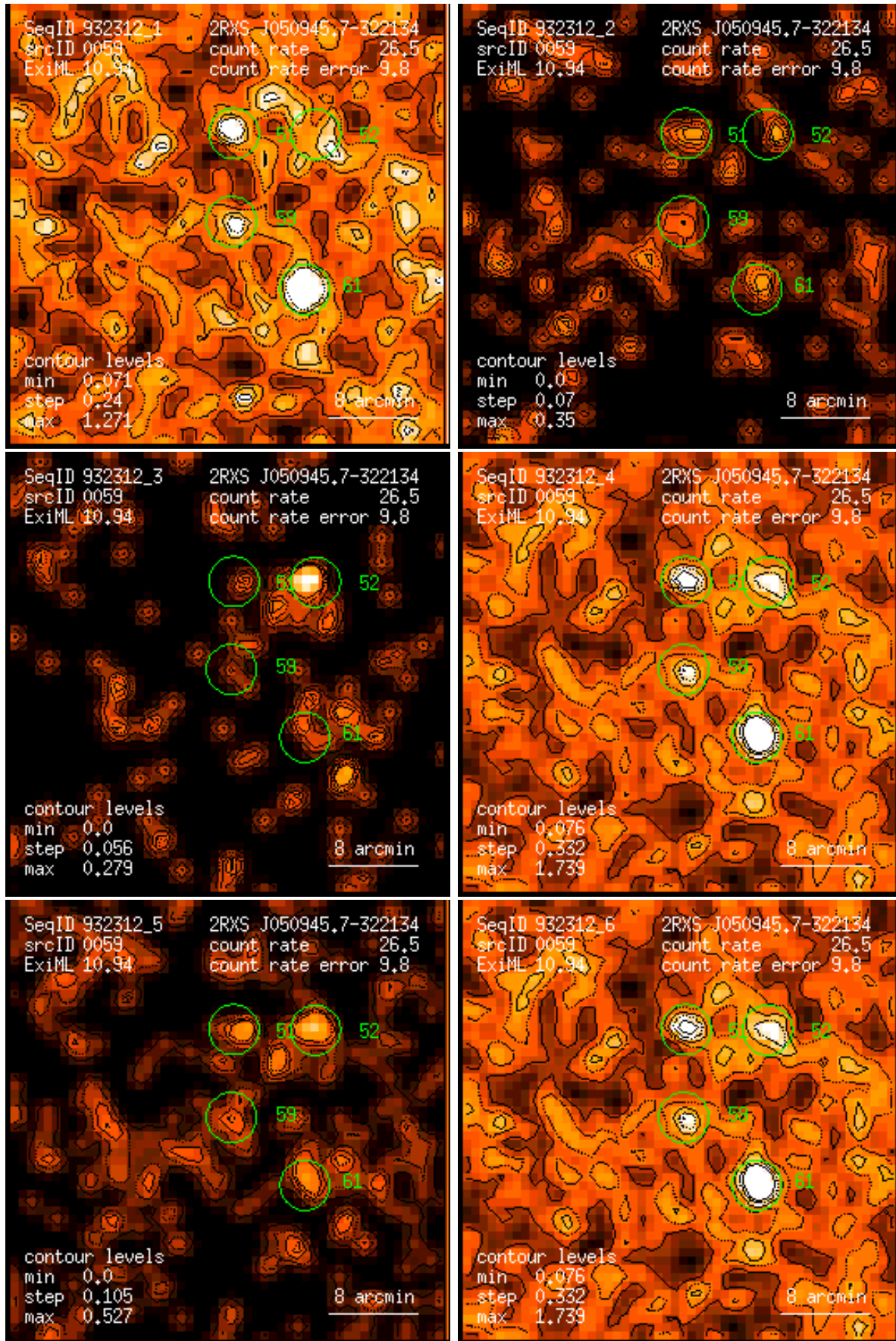
Figure 59: RASS 932312: detection 0059: band rate images, Gaussian filter: (1) PSPC channels 11 – 41, (2) 52 – 90, (3) 91 – 201, (4) 11 – 235, (5) 52 – 201, (6) 11 – 201. Broad band rates in counts/ks. Band rate contour levels in counts/ks/arcmin 2 .
