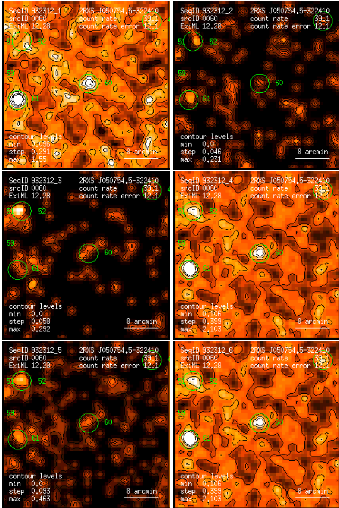
Figure 60: RASS 932312: detection 0060: band rate images, Gaussian filter: (1) PSPC channels 11 – 41, (2) 52 – 90, (3) 91 – 201, (4) 11 – 235, (5) 52 – 201, (6) 11 – 201. Broad band rates in counts/ks. Band rate contour levels in counts/ks/arcmin 2 .
