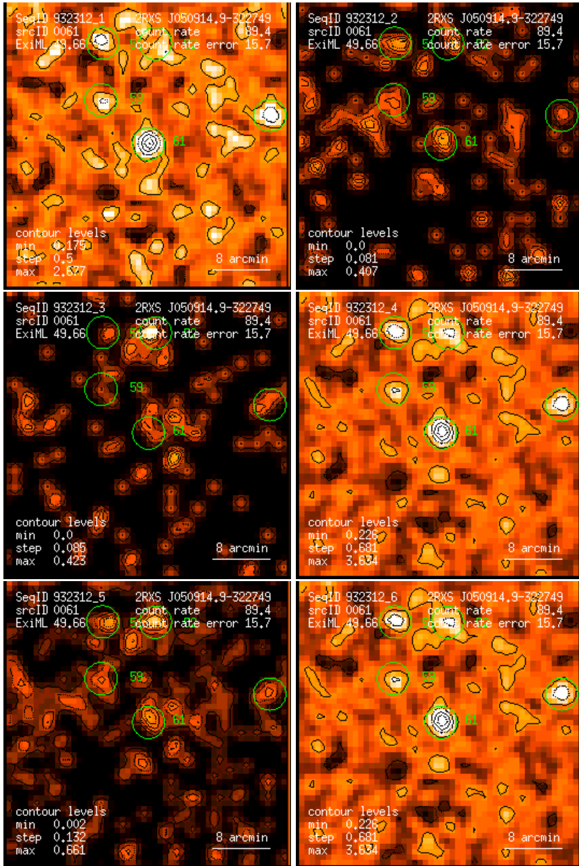
Figure 61: RASS 932312: detection 0061: band rate images, Gaussian filter: (1) PSPC channels 11 – 41, (2) 52 – 90, (3) 91 – 201, (4) 11 – 235, (5) 52 – 201, (6) 11 – 201. Broad band rates in counts/ks. Band rate contour levels in counts/ks/arcmin 2 .
