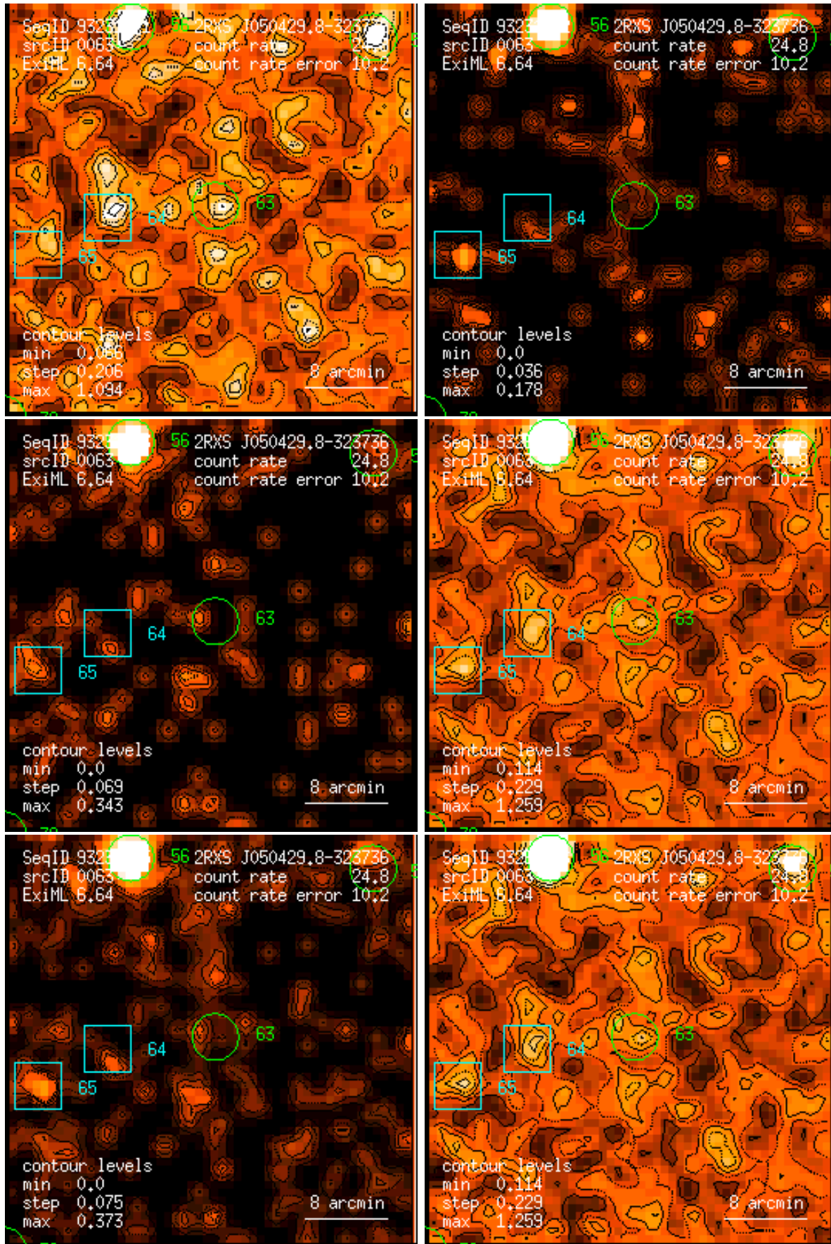
Figure 63: RASS 932312: detection 0063: band rate images, Gaussian filter: (1) PSPC channels 11 – 41, (2) 52 – 90, (3) 91 – 201, (4) 11 – 235, (5) 52 – 201, (6) 11 – 201. Broad band rates in counts/ks. Band rate contour levels in counts/ks/arcmin 2 .
