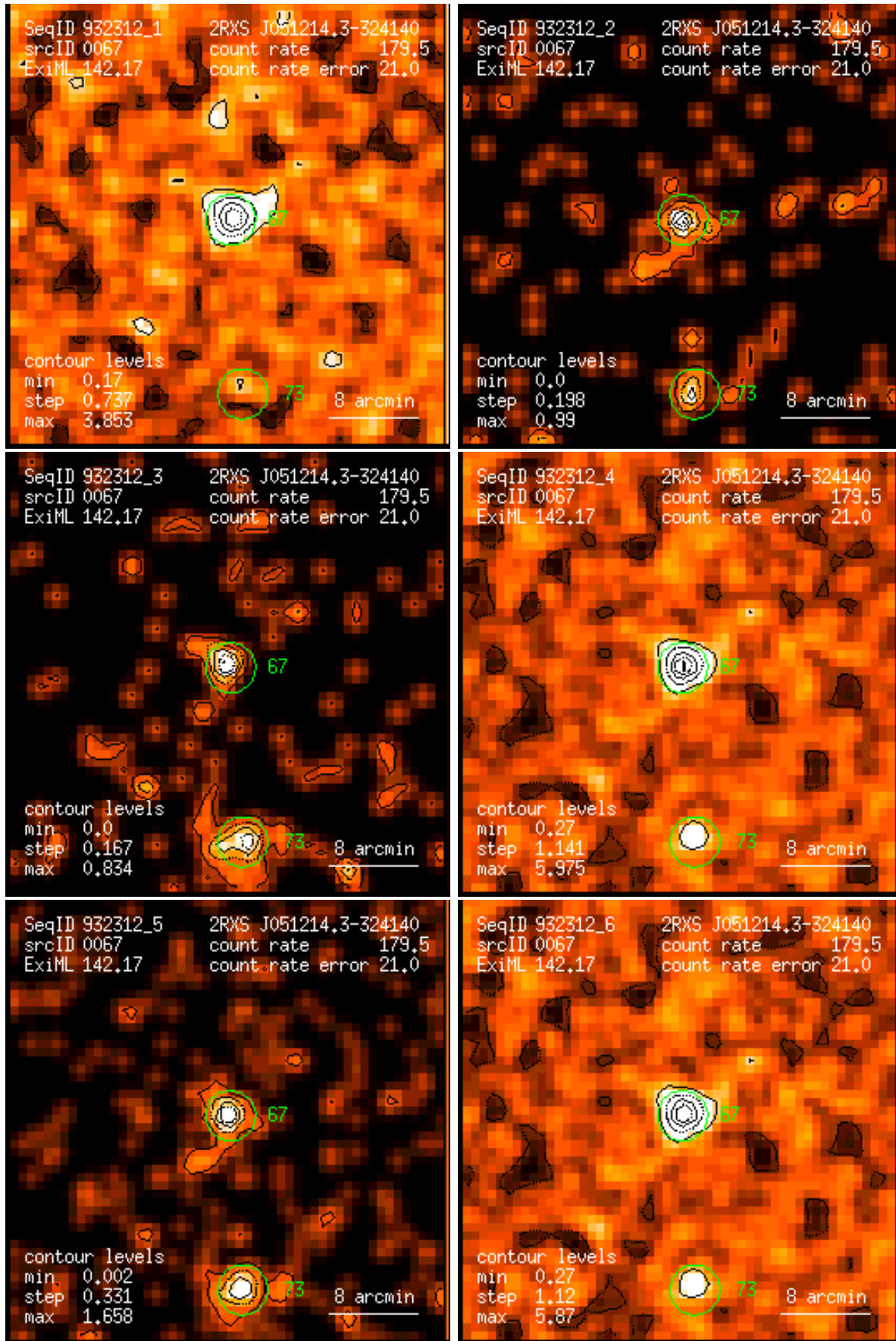
Figure 67: RASS 932312: detection 0067: band rate images, Gaussian filter: (1) PSPC channels 11 – 41, (2) 52 – 90, (3) 91 – 201, (4) 11 – 235, (5) 52 – 201, (6) 11 – 201. Broad band rates in counts/ks. Band rate contour levels in counts/ks/arcmin 2 .
