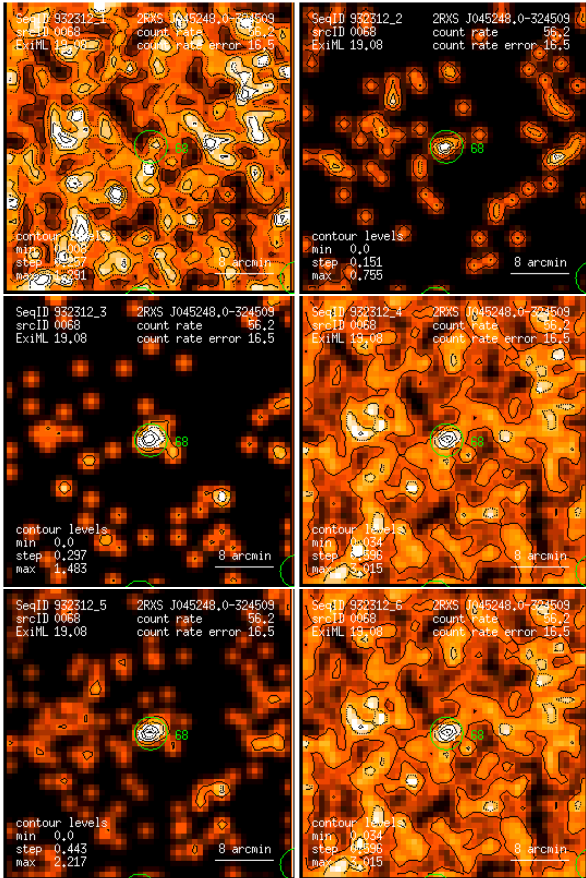
Figure 68: RASS 932312: detection 0068: band rate images, Gaussian filter: (1) PSPC channels 11 – 41, (2) 52 – 90, (3) 91 – 201, (4) 11 – 235, (5) 52 – 201, (6) 11 – 201. Broad band rates in counts/ks. Band rate contour levels in counts/ks/arcmin 2 .
