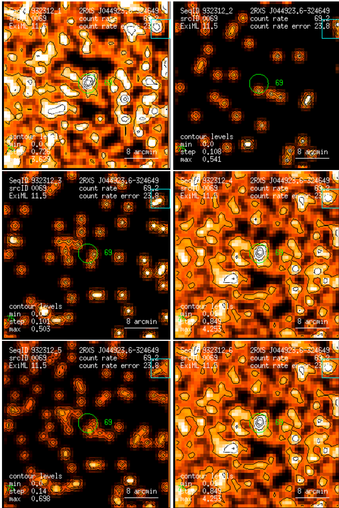
Figure 69: RASS 932312: detection 0069: band rate images, Gaussian filter: (1) PSPC channels 11 – 41, (2) 52 – 90, (3) 91 – 201, (4) 11 – 235, (5) 52 – 201, (6) 11 – 201. Broad band rates in counts/ks. Band rate contour levels in counts/ks/arcmin 2 .
