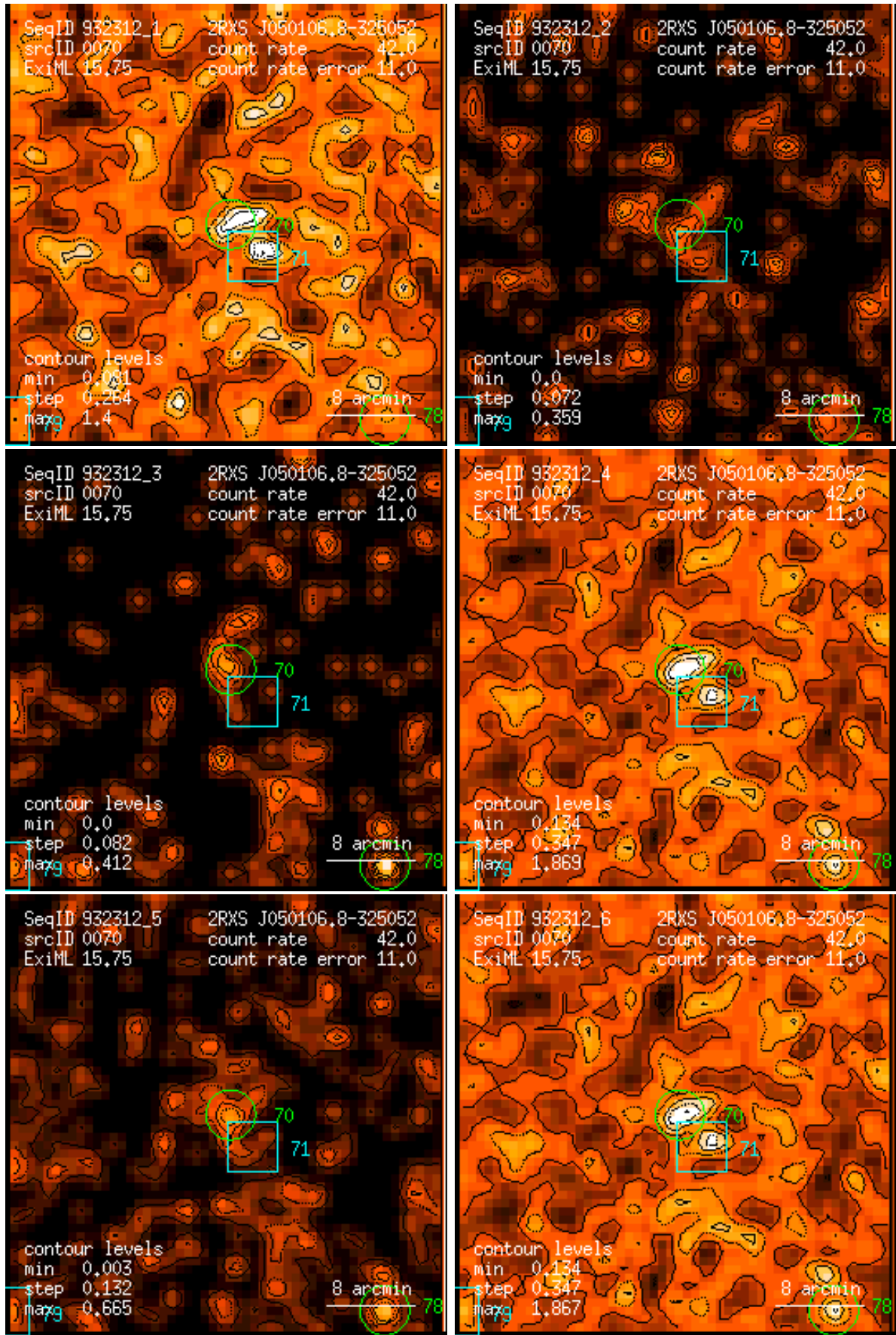
Figure 70: RASS 932312: detection 0070: band rate images, Gaussian filter: (1) PSPC channels 11 – 41, (2) 52 – 90, (3) 91 – 201, (4) 11 – 235, (5) 52 – 201, (6) 11 – 201. Broad band rates in counts/ks. Band rate contour levels in counts/ks/arcmin 2 .
