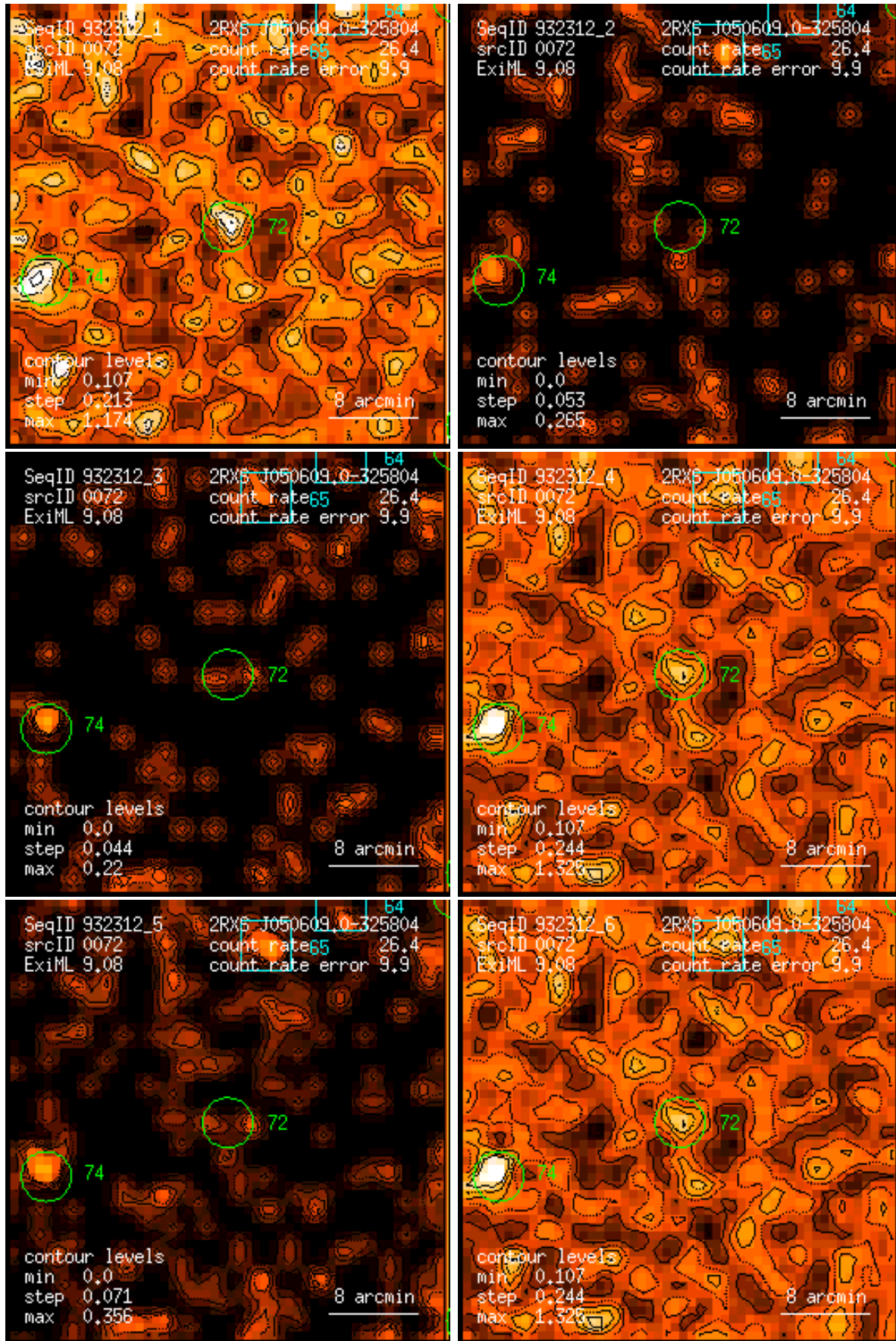
Figure 72: RASS 932312: detection 0072: band rate images, Gaussian filter: (1) PSPC channels 11 – 41, (2) 52 – 90, (3) 91 – 201, (4) 11 – 235, (5) 52 – 201, (6) 11 – 201. Broad band rates in counts/ks. Band rate contour levels in counts/ks/arcmin 2 .
