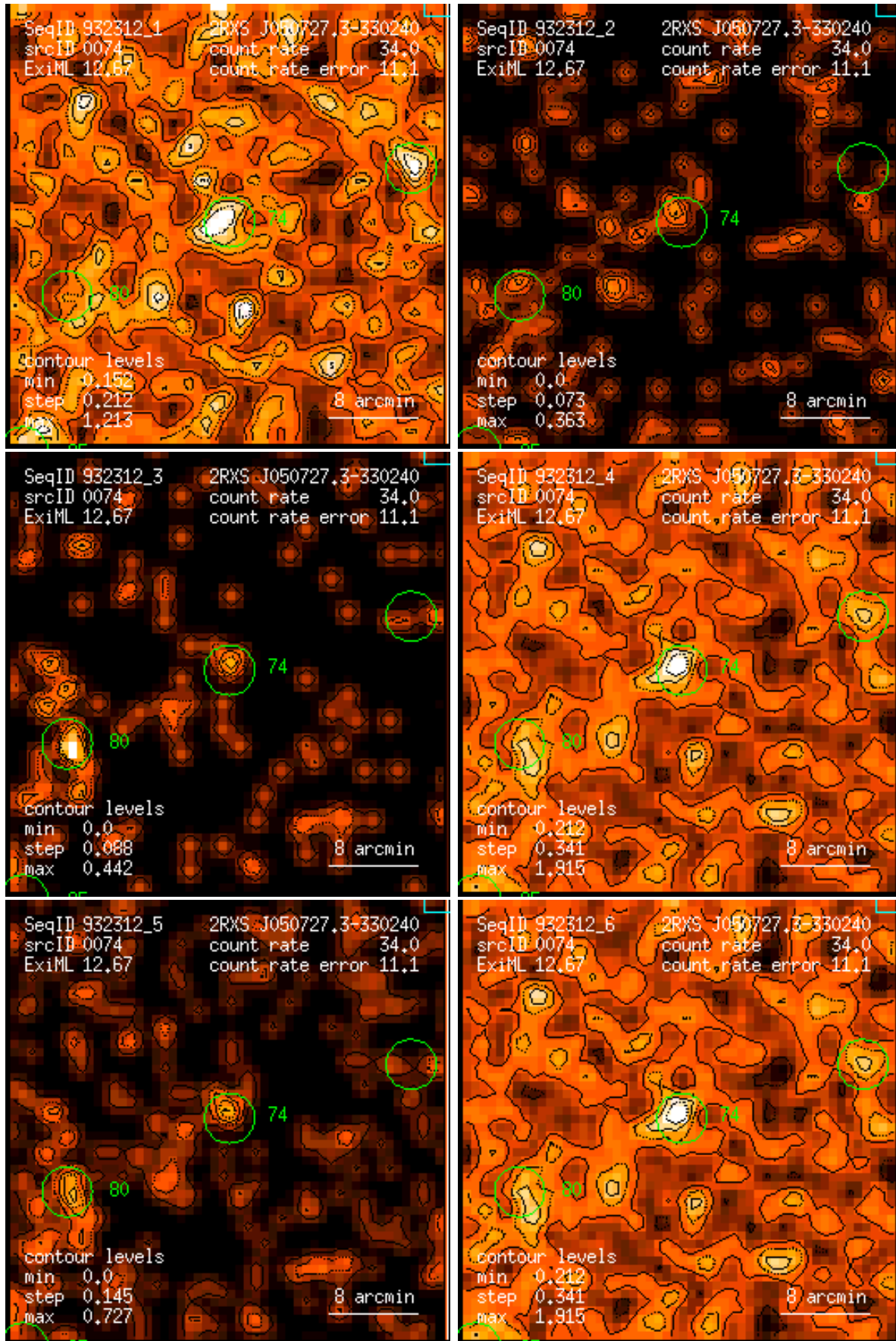
Figure 74: RASS 932312: detection 0074: band rate images, Gaussian filter: (1) PSPC channels 11 – 41, (2) 52 – 90, (3) 91 – 201, (4) 11 – 235, (5) 52 – 201, (6) 11 – 201. Broad band rates in counts/ks. Band rate contour levels in counts/ks/arcmin 2 .
