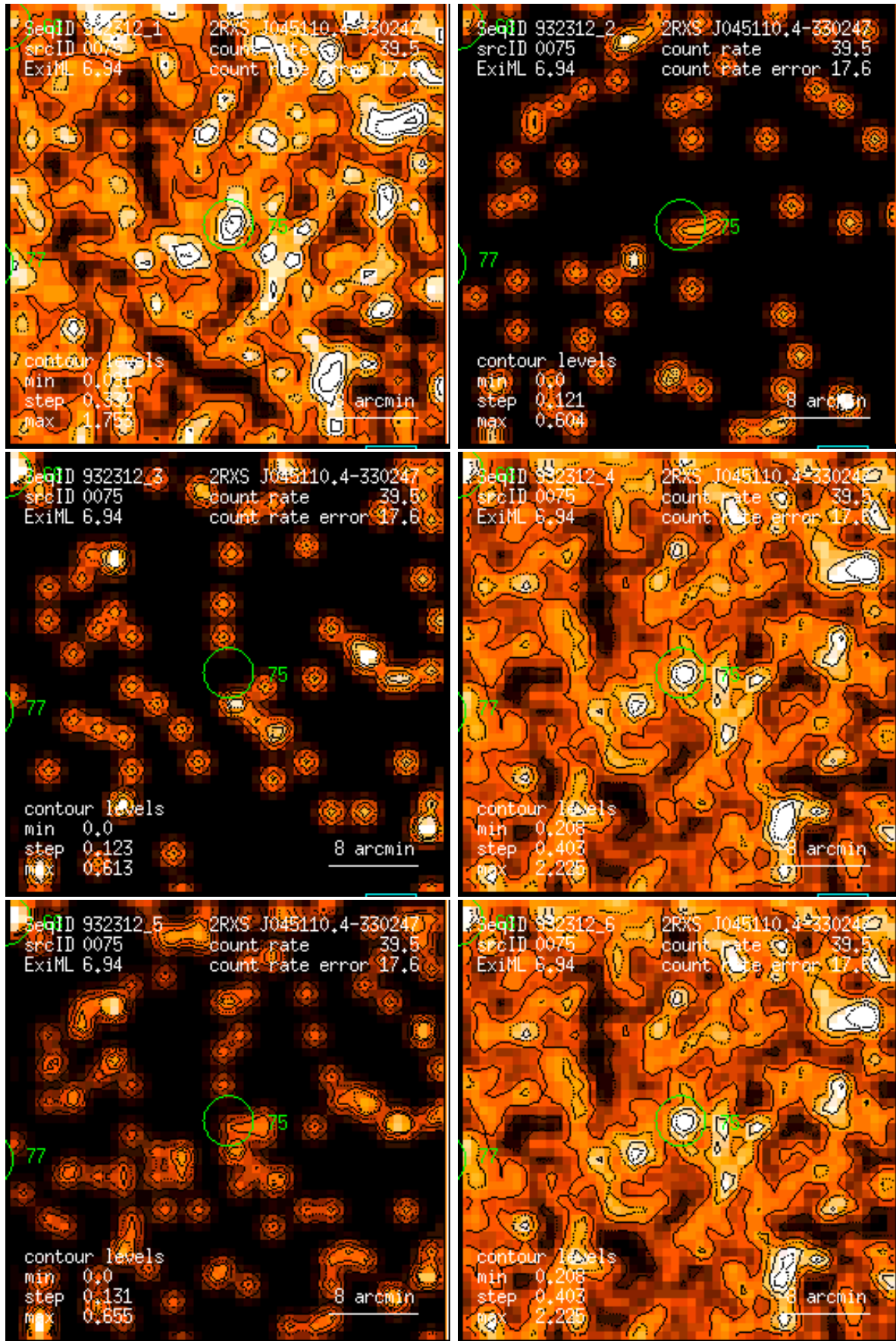
Figure 75: RASS 932312: detection 0075: band rate images, Gaussian filter: (1) PSPC channels 11 – 41, (2) 52 – 90, (3) 91 – 201, (4) 11 – 235, (5) 52 – 201, (6) 11 – 201. Broad band rates in counts/ks. Band rate contour levels in counts/ks/arcmin 2 .
