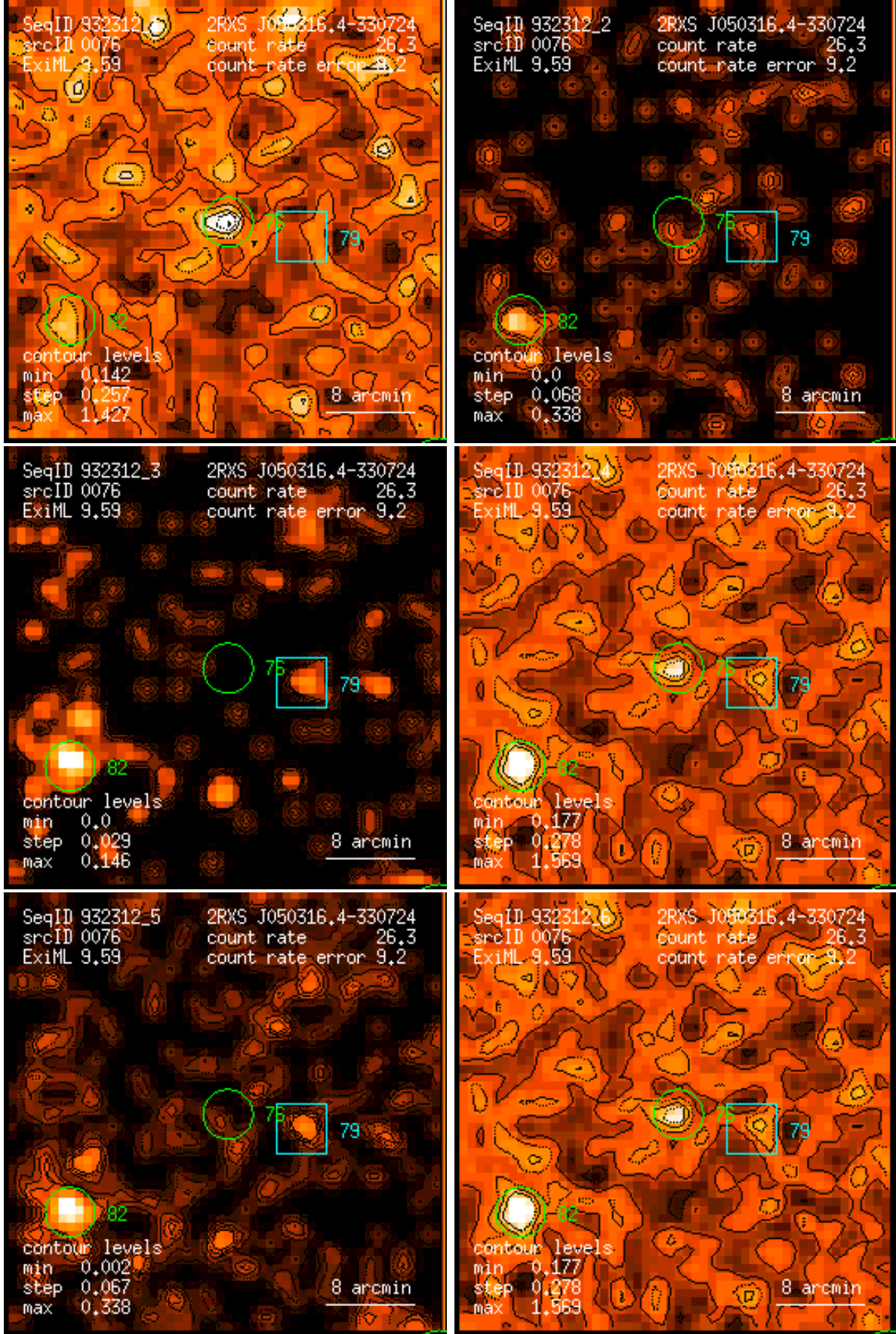
Figure 76: RASS 932312: detection 0076: band rate images, Gaussian filter: (1) PSPC channels 11 – 41, (2) 52 – 90, (3) 91 – 201, (4) 11 – 235, (5) 52 – 201, (6) 11 – 201. Broad band rates in counts/ks. Band rate contour levels in counts/ks/arcmin 2 .
