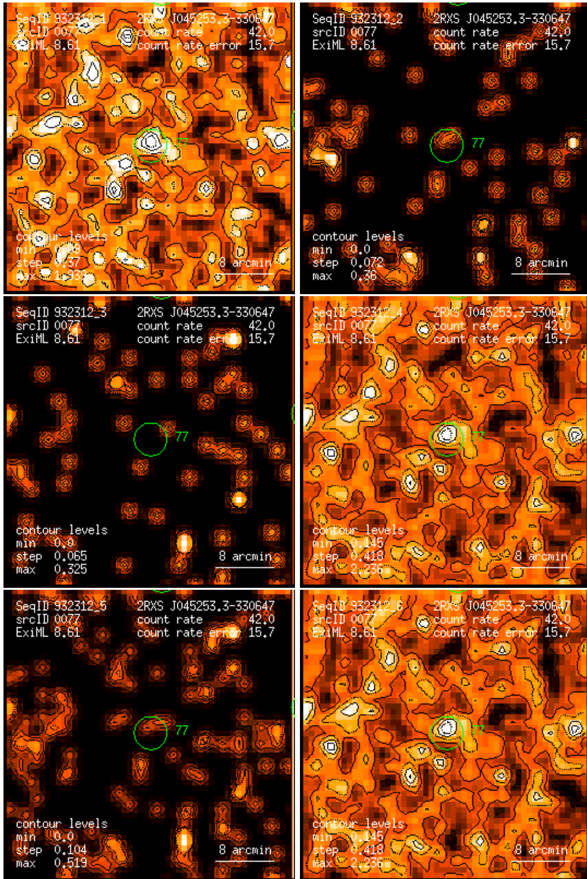
Figure 77: RASS 932312: detection 0077: band rate images, Gaussian filter: (1) PSPC channels 11 – 41, (2) 52 – 90, (3) 91 – 201, (4) 11 – 235, (5) 52 – 201, (6) 11 – 201. Broad band rates in counts/ks. Band rate contour levels in counts/ks/arcmin 2 .
