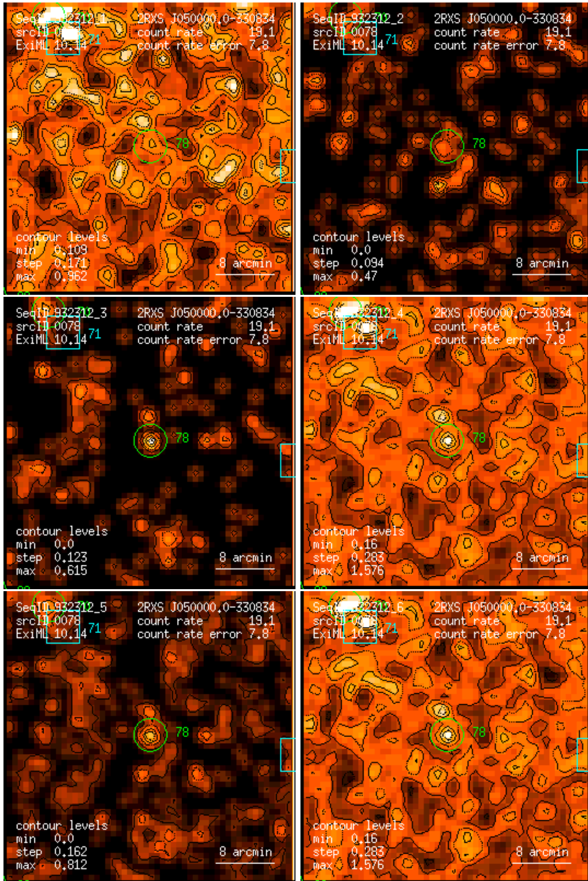
Figure 78: RASS 932312: detection 0078: band rate images, Gaussian filter: (1) PSPC channels 11 – 41, (2) 52 – 90, (3) 91 – 201, (4) 11 – 235, (5) 52 – 201, (6) 11 – 201. Broad band rates in counts/ks. Band rate contour levels in counts/ks/arcmin 2 .
