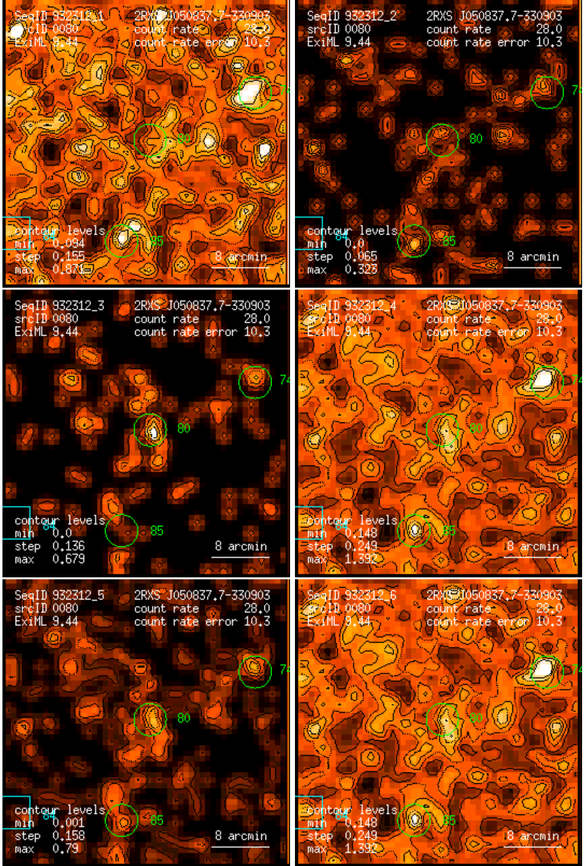
Figure 80: RASS 932312: detection 0080: band rate images, Gaussian filter: (1) PSPC channels 11 – 41, (2) 52 – 90, (3) 91 – 201, (4) 11 – 235, (5) 52 – 201, (6) 11 – 201. Broad band rates in counts/ks. Band rate contour levels in counts/ks/arcmin 2 .
