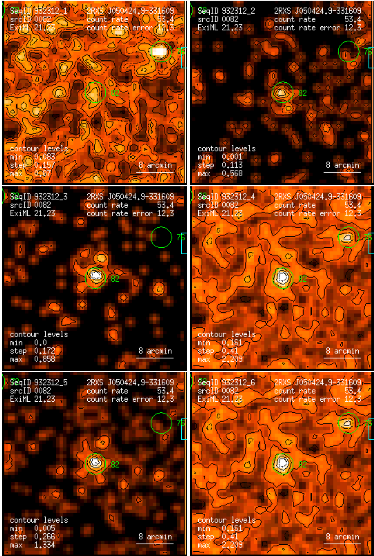
Figure 82: RASS 932312: detection 0082: band rate images, Gaussian filter: (1) PSPC channels 11 – 41, (2) 52 – 90, (3) 91 – 201, (4) 11 – 235, (5) 52 – 201, (6) 11 – 201. Broad band rates in counts/ks. Band rate contour levels in counts/ks/arcmin 2 .
