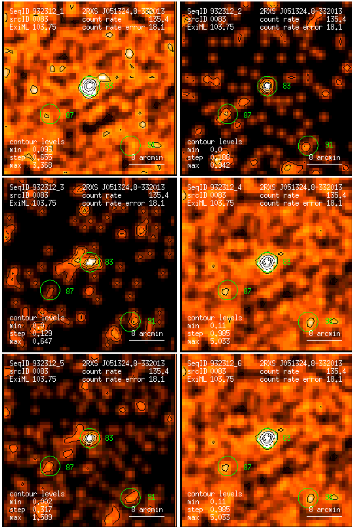
Figure 83: RASS 932312: detection 0083: band rate images, Gaussian filter: (1) PSPC channels 11 – 41, (2) 52 – 90, (3) 91 – 201, (4) 11 – 235, (5) 52 – 201, (6) 11 – 201. Broad band rates in counts/ks. Band rate contour levels in counts/ks/arcmin 2 .
