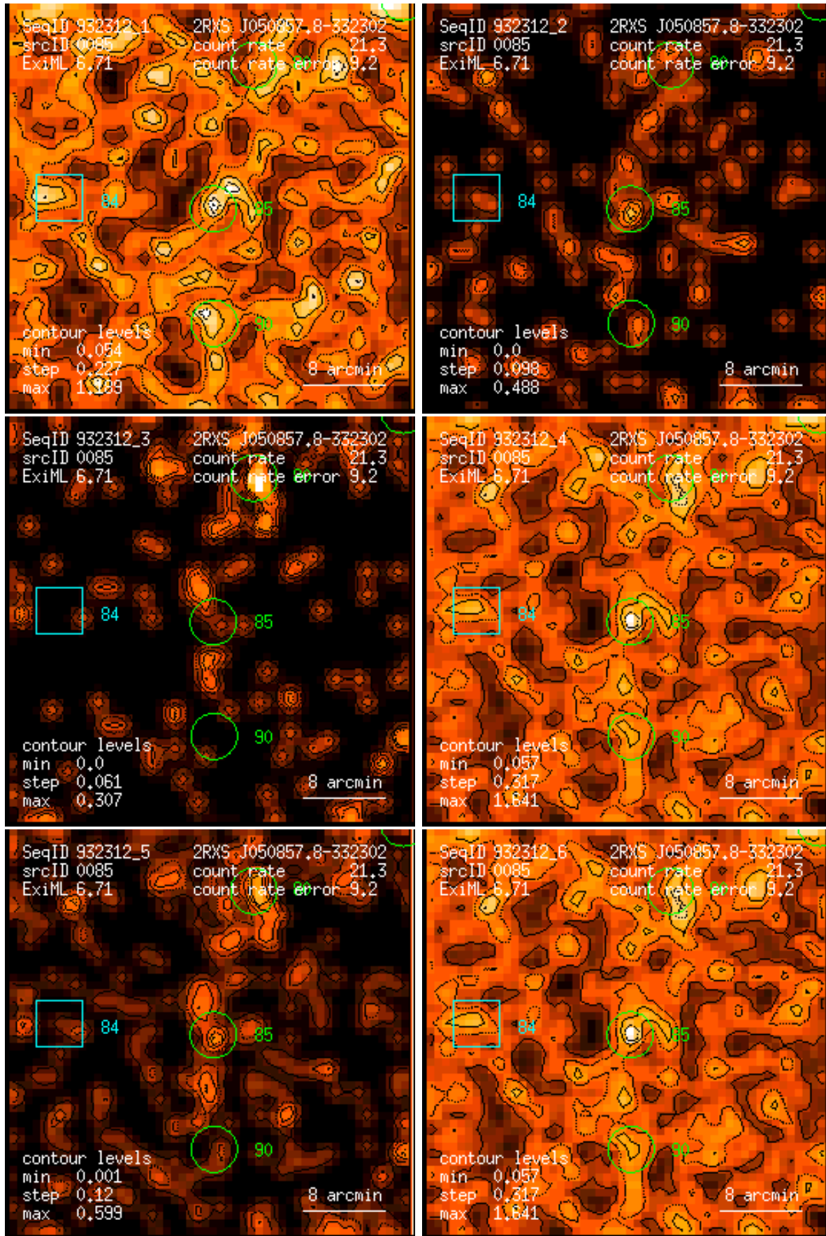
Figure 85: RASS 932312: detection 0085: band rate images, Gaussian filter: (1) PSPC channels 11 – 41, (2) 52 – 90, (3) 91 – 201, (4) 11 – 235, (5) 52 – 201, (6) 11 – 201. Broad band rates in counts/ks. Band rate contour levels in counts/ks/arcmin 2 .
