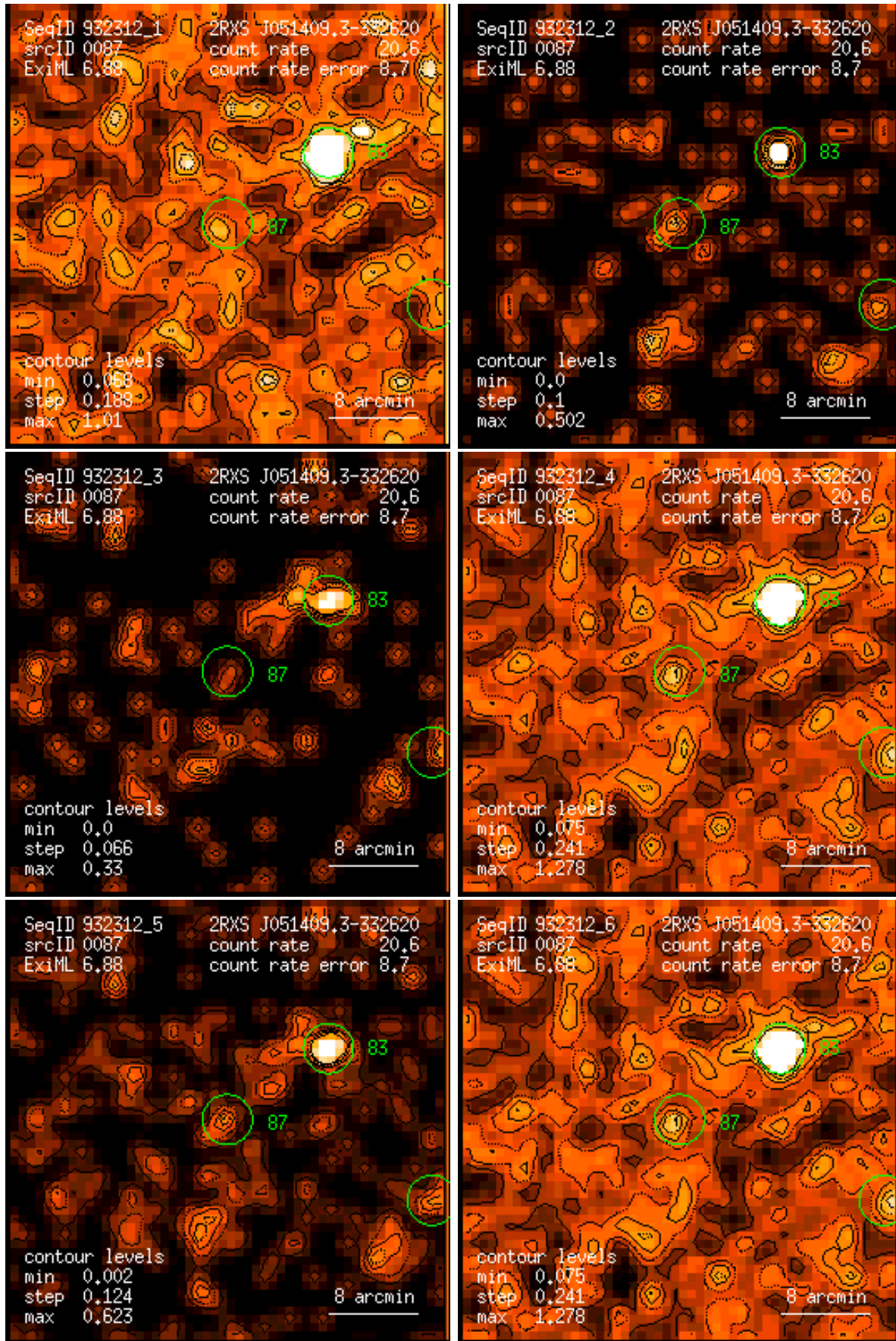
Figure 87: RASS 932312: detection 0087: band rate images, Gaussian filter: (1) PSPC channels 11 – 41, (2) 52 – 90, (3) 91 – 201, (4) 11 – 235, (5) 52 – 201, (6) 11 – 201. Broad band rates in counts/ks. Band rate contour levels in counts/ks/arcmin 2 .
