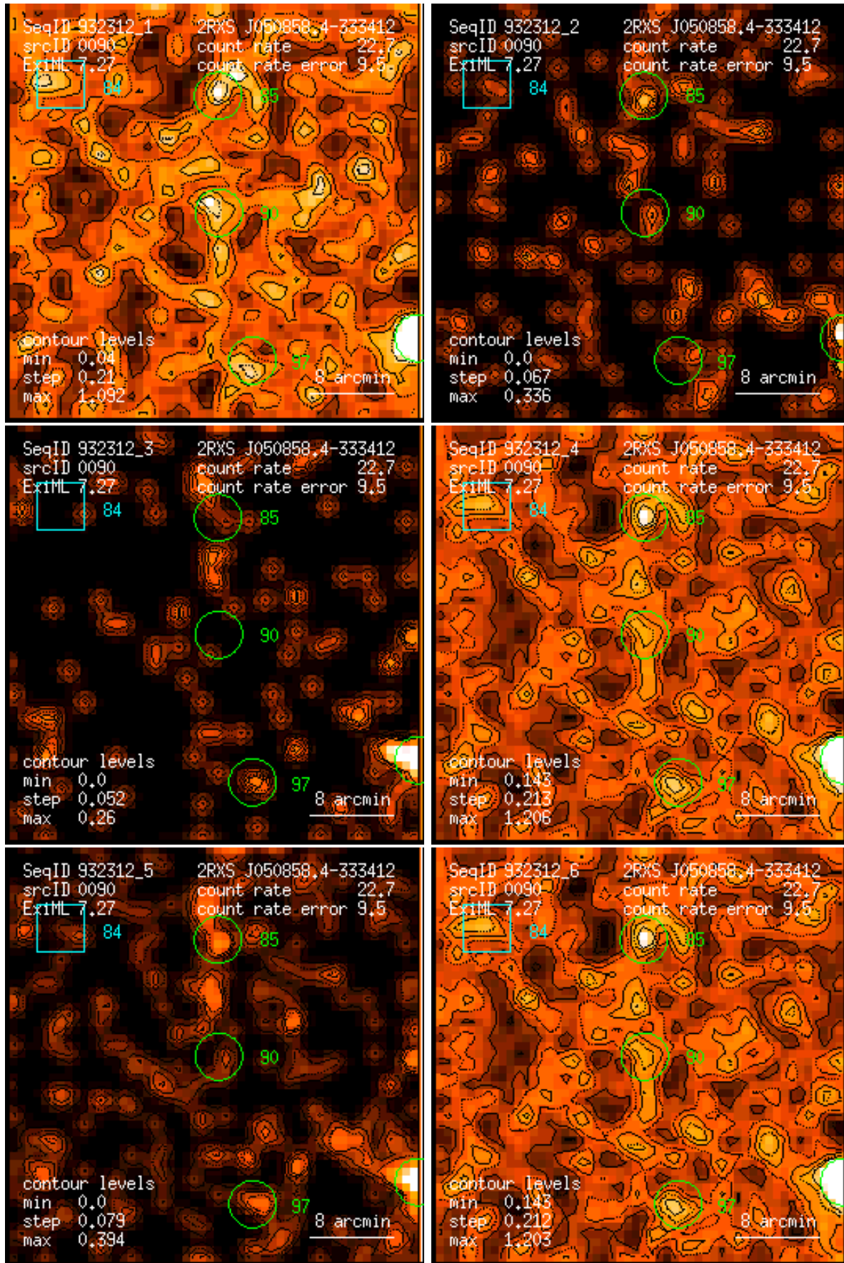
Figure 90: RASS 932312: detection 0090: band rate images, Gaussian filter: (1) PSPC channels 11 – 41, (2) 52 – 90, (3) 91 – 201, (4) 11 – 235, (5) 52 – 201, (6) 11 – 201. Broad band rates in counts/ks. Band rate contour levels in counts/ks/arcmin 2 .
