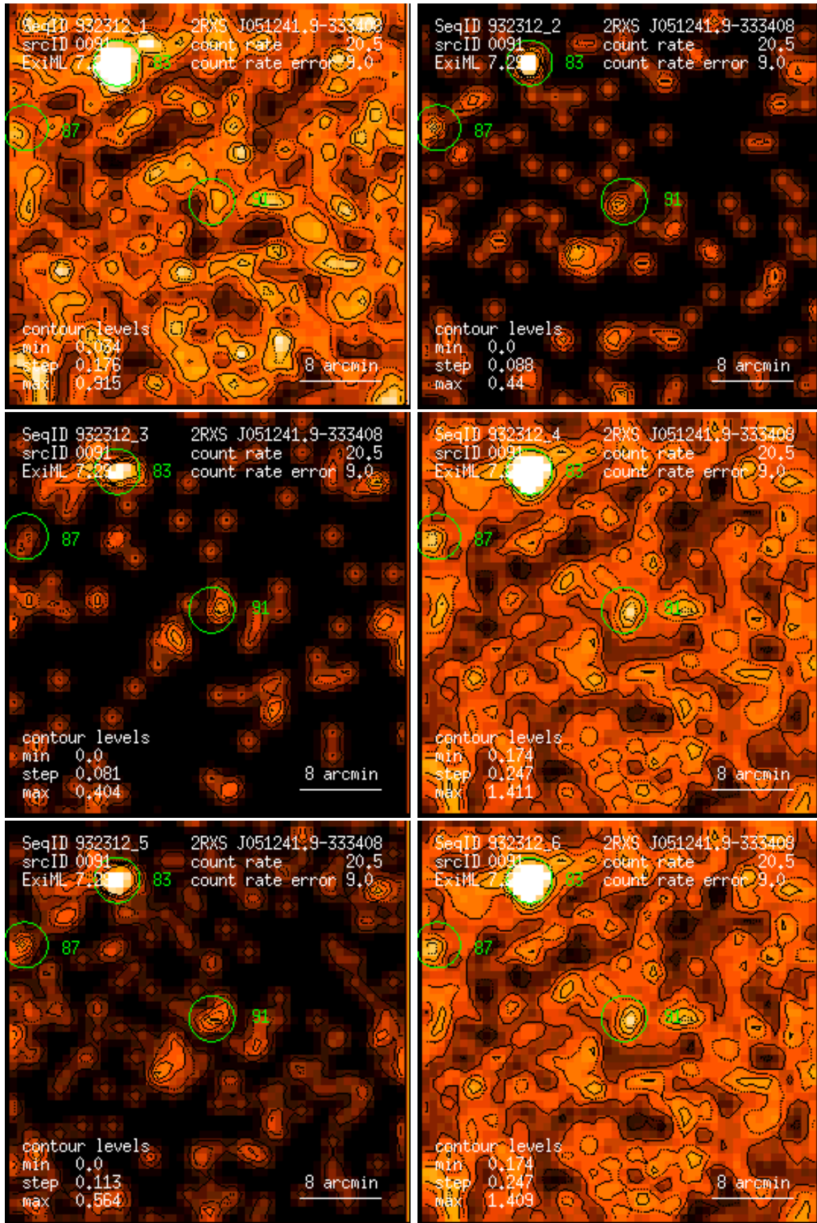
Figure 91: RASS 932312: detection 0091: band rate images, Gaussian filter: (1) PSPC channels 11 – 41, (2) 52 – 90, (3) 91 – 201, (4) 11 – 235, (5) 52 – 201, (6) 11 – 201. Broad band rates in counts/ks. Band rate contour levels in counts/ks/arcmin 2 .
