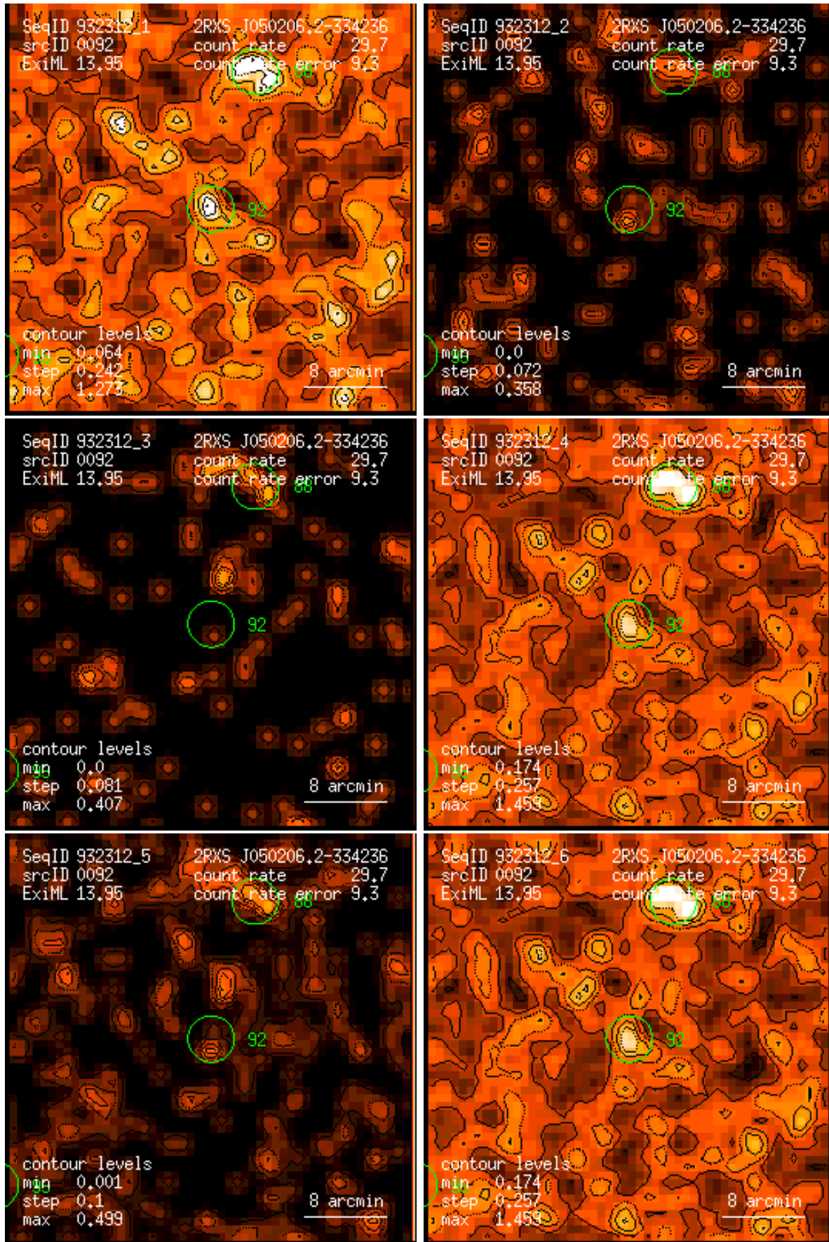
Figure 92: RASS 932312: detection 0092: band rate images, Gaussian filter: (1) PSPC channels 11 – 41, (2) 52 – 90, (3) 91 – 201, (4) 11 – 235, (5) 52 – 201, (6) 11 – 201. Broad band rates in counts/ks. Band rate contour levels in counts/ks/arcmin 2 .
